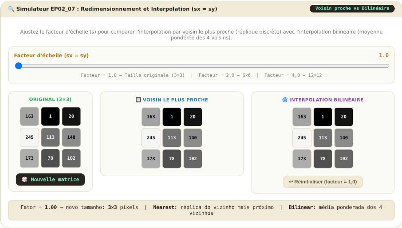
Versão interativa: https://fzampirolli.github.io/pdi-vc/simuladores/cpp.fr/cap02/sim-ep0207-escala.html Figure 2.18: Simulateur EP02_07 : Redimensionnement spatial et interpolation (Nearest Neighbor vs Bilinéaire)
