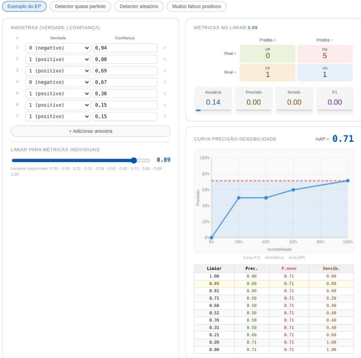
Figura 1.14: Simulador: Mean Average Precision (mAP) - Curva P-S
