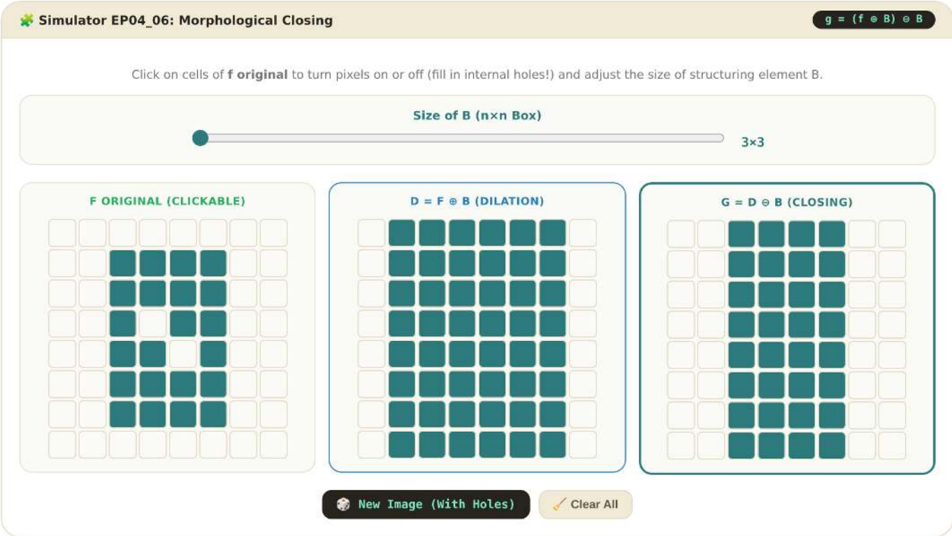
Figure 4.35: EP04_06 Simulator: Morphological Closing ( g = (f \oplus B) \odot B )
