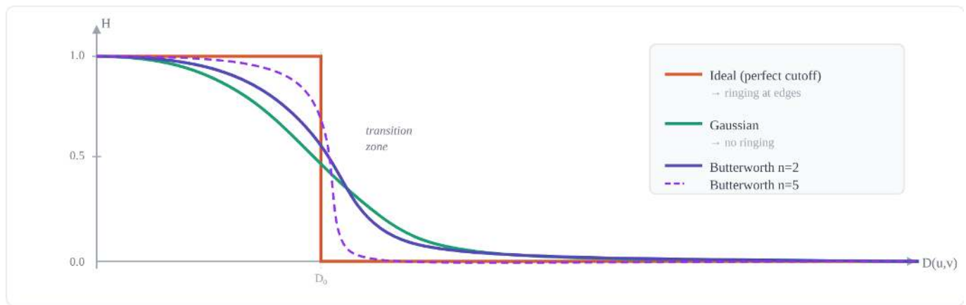
Figure 5.11: Low-pass filters.
