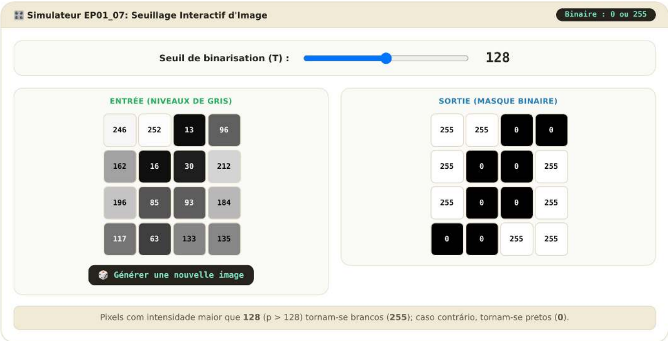
Versão interativa: https://fzampirolli.github.io/pdi-vc/simuladores/cpp.fr/cap01/sim-ep0107-limiarizacao.html Figure 1.17: Simulateur EP01_07 : Seuillage global interactif (binarisation p > T )
