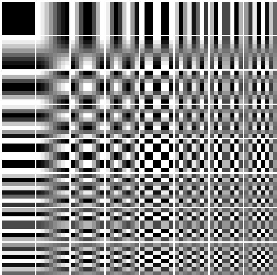
As 64 Bases da DCT 8x8
