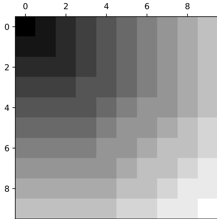
mm.dist (L2)
