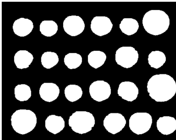
4. Opening (cleaning)
