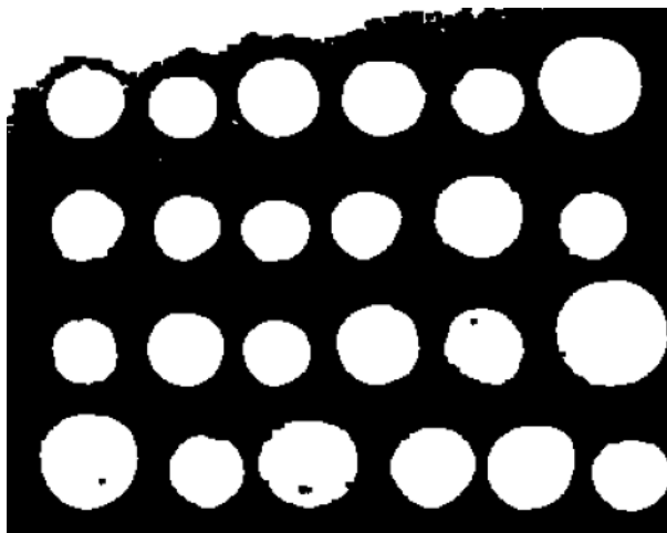
1. Thresholding (Otsu)
