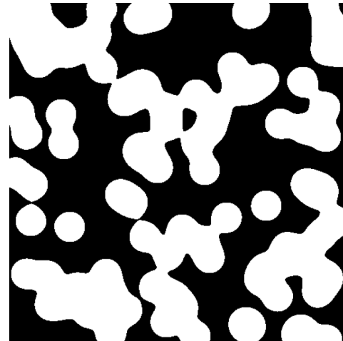
binary_blobs
