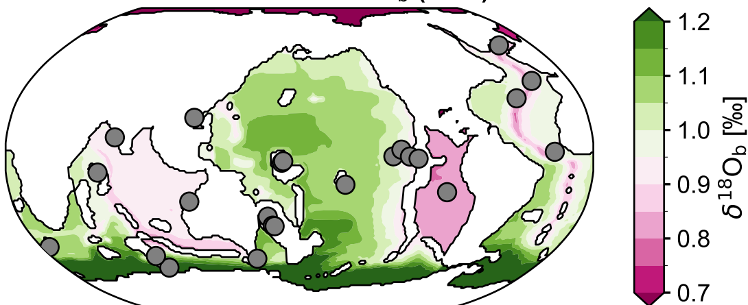
c Predicted Bottom \delta^{18}\text{O}_b (MLE)
