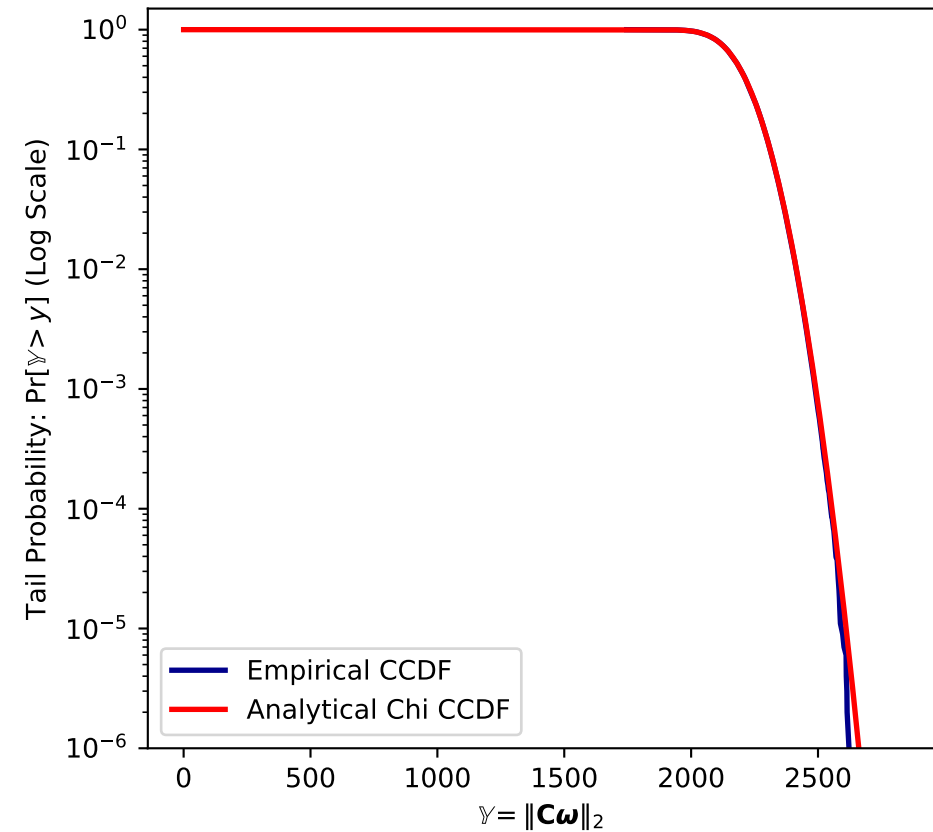
Log-Scale Tail (CCDF) Comparison
