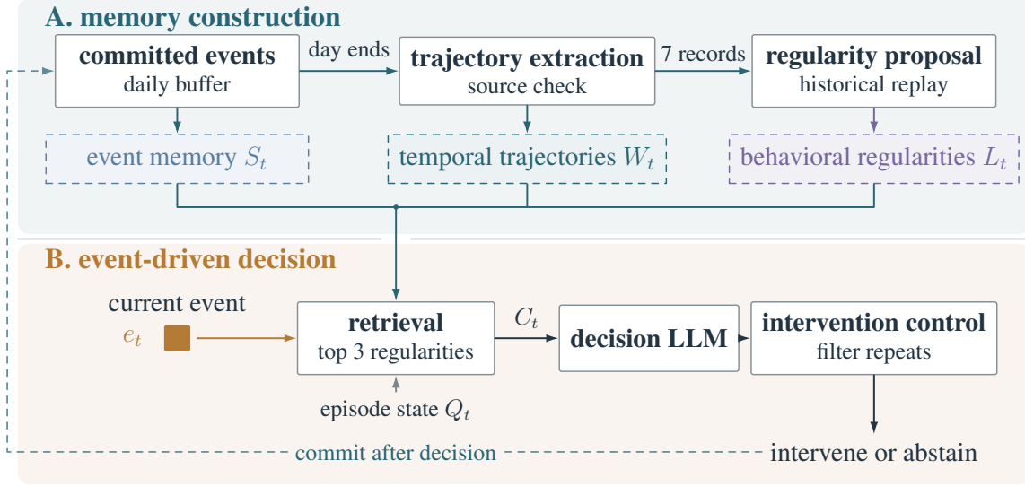
Figure 2: ProactMem architecture. (A) Completed history supplies bounded events; construction LLMs produce source-checked temporal trajectories and replay-assessed behavioral regularities. (B) The current event guides retrieval of up to three applicable regularities. Context C_t combines these regularities with recent events, temporal trajectories, the current event, and episode state Q_t . The decision LLM proposes assistance, intervention control filters repetition, and dashed feedback commits the event after finalization.
