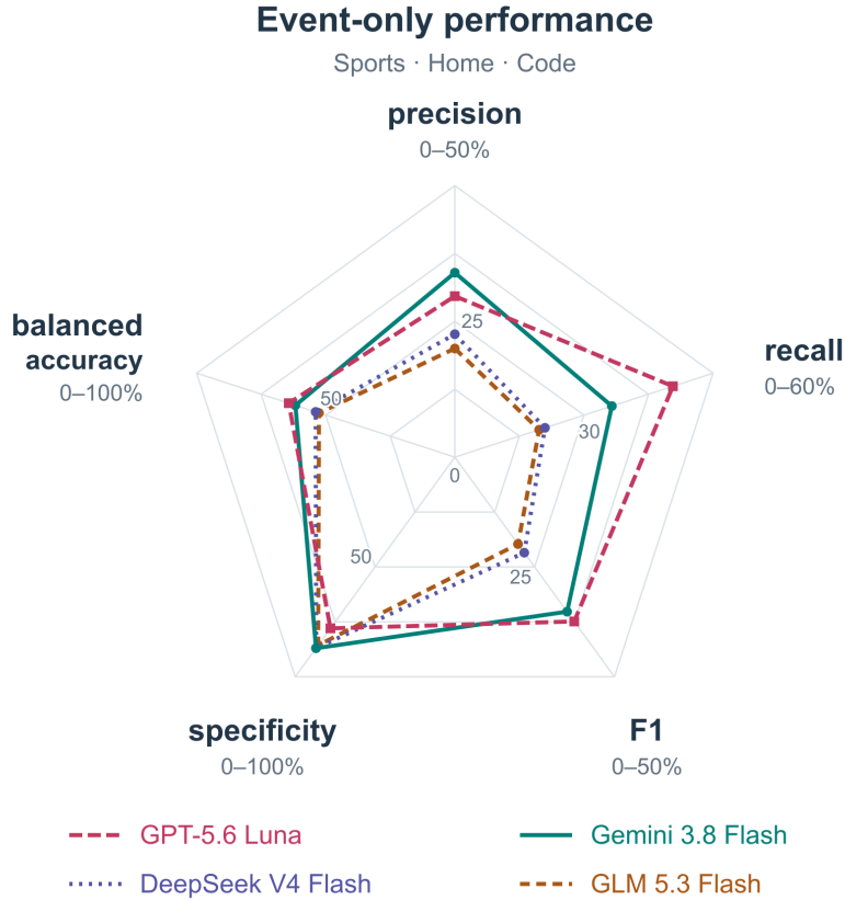
Figure 4: Single-run event-only model comparison on three selected streams. Scores pool event-level confusion counts across domains; specificity equals 1 - \text{intrusion} . All axes start at zero, with metric-specific ranges.
