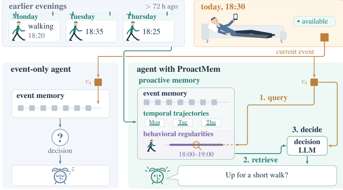
Figure 1: Illustrative Sports scenario. Both agents receive the same current event and recent history. The current event queries ProactMem to match stored behavioral regularities. Retrieved regularities join recent events and temporal trajectories in the decision context. Responses depict possible decisions.
