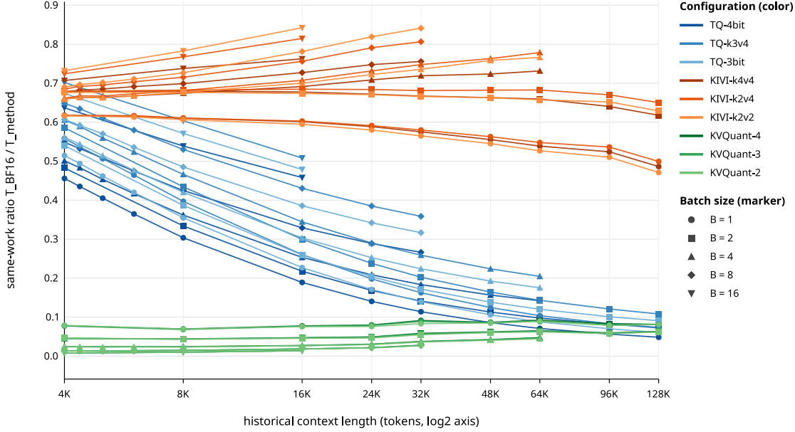
Figure 1. Wall-clock same-work ratio T_{\text{BF16}}/T_{\text{method}} versus historical context in Graph mode, one line per compressed configuration (color) and batch size (marker). Every ratio is below 1.
