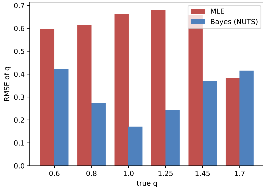
(b) Strong truncation: RMSE by q
