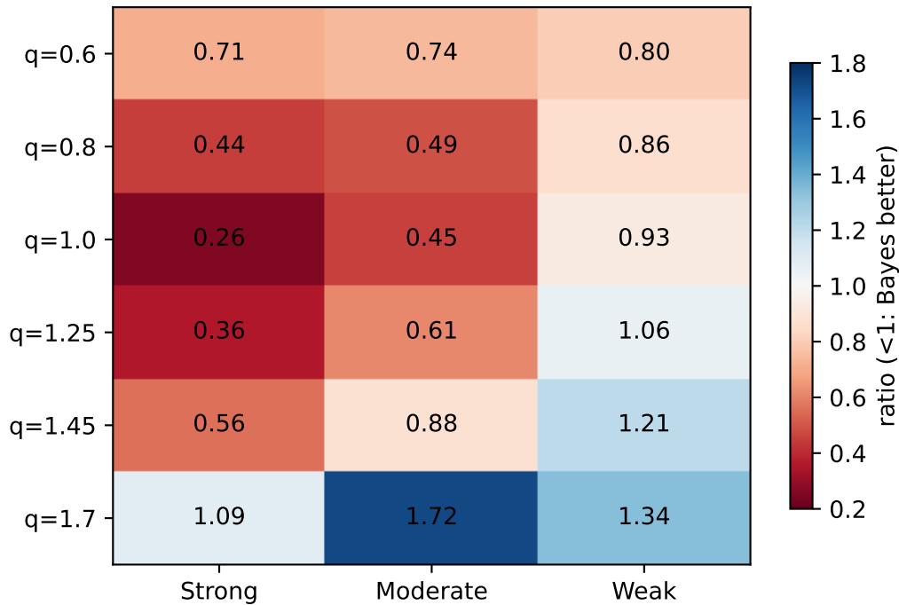
(a) RMSE ratio Bayes / MLE
