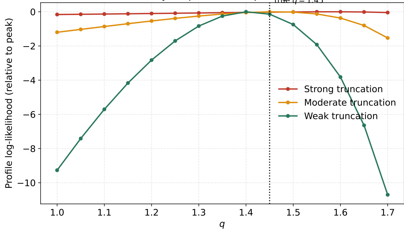
Identifiability of q under competing truncation
