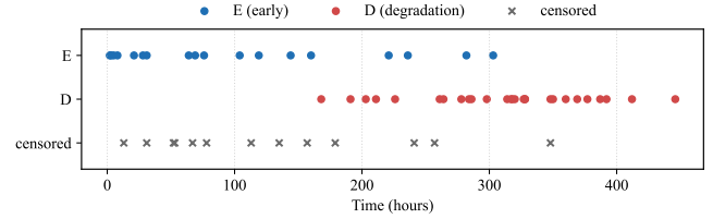
FIGURE 7 | Event and censoring times by failure mode for the voltage data.
