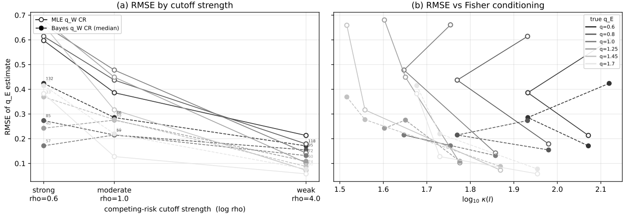
FIGURE 2 | Weak-identifiability map. Across true q , the observed information ( \det \mathbf{I} , smallest eigenvalue \lambda_{\min} , condition number \kappa ) and the target-cause event fraction \text{frac}_{\text{event}} improve monotonically as truncation weakens, and the MLE RMSE( q ) tracks the resulting information scarcity. MLE RMSE: open circles, solid line; Bayes RMSE: filled circles, dashed line.
