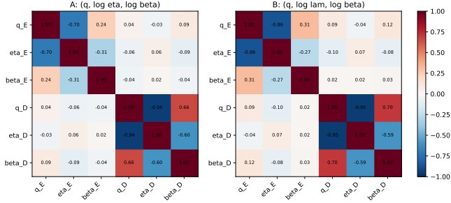
FIGURE 1 | Posterior correlation structure (parametric comparison). The alternative (q, \log \lambda, \log \beta) parameterisation (B) is not more orthogonal: its Hessian is about 550 times worse-conditioned and its chains fail to converge. We therefore retain (q, \log \eta, \log \beta) and describe it only as a better-conditioned, unconstrained system.
