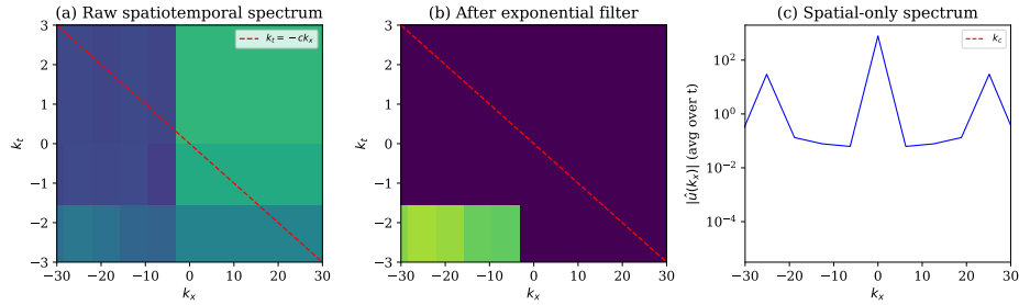
Figure 3: Spatiotemporal spectrum of the advection solution. (a) Raw 2D Fourier transform: energy concentrates along the characteristic line “ k_t = -ck_x ” (red dashed). (b) After exponential filtering: high-frequency boundary ringing is suppressed. (c) Spatial-only spectrum averaged over time: the broad, slowly decaying profile reflects Gibbs ringing from the non-periodic boundary.
