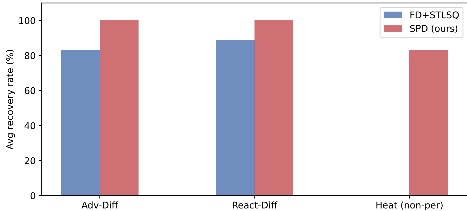
2D PDE recovery (pointwise variant)
