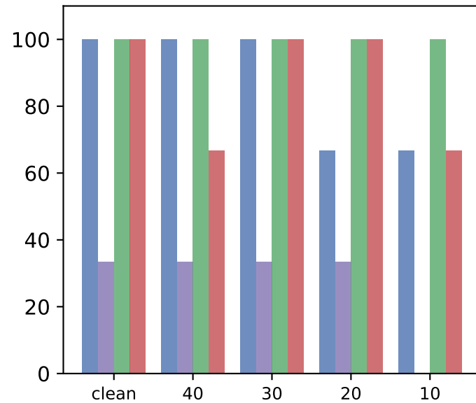
KS
