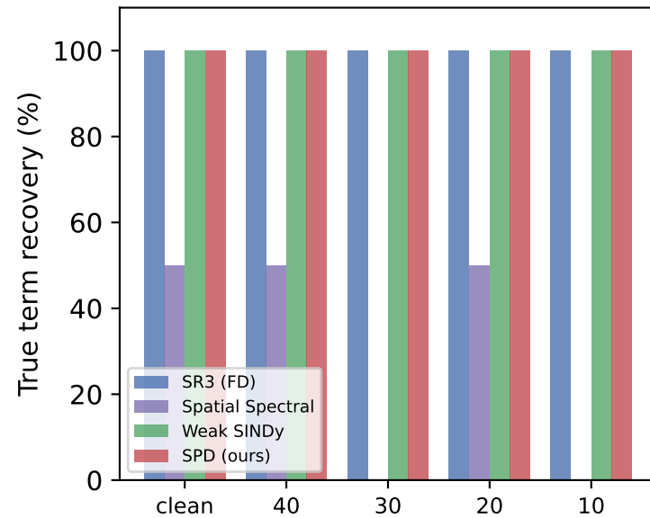
Burgers
