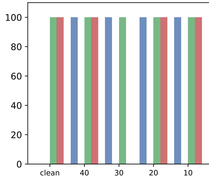
Advection
