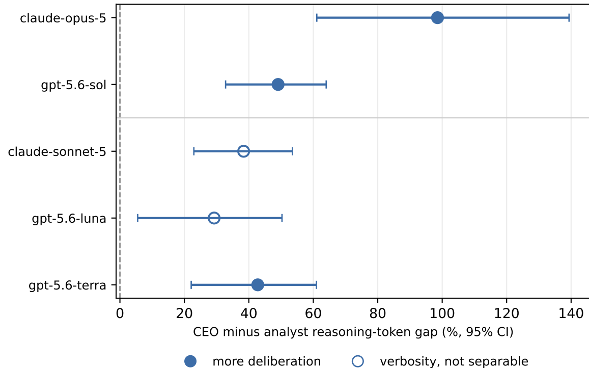
Does the model reason more when it believes it is talking to the CEO?
