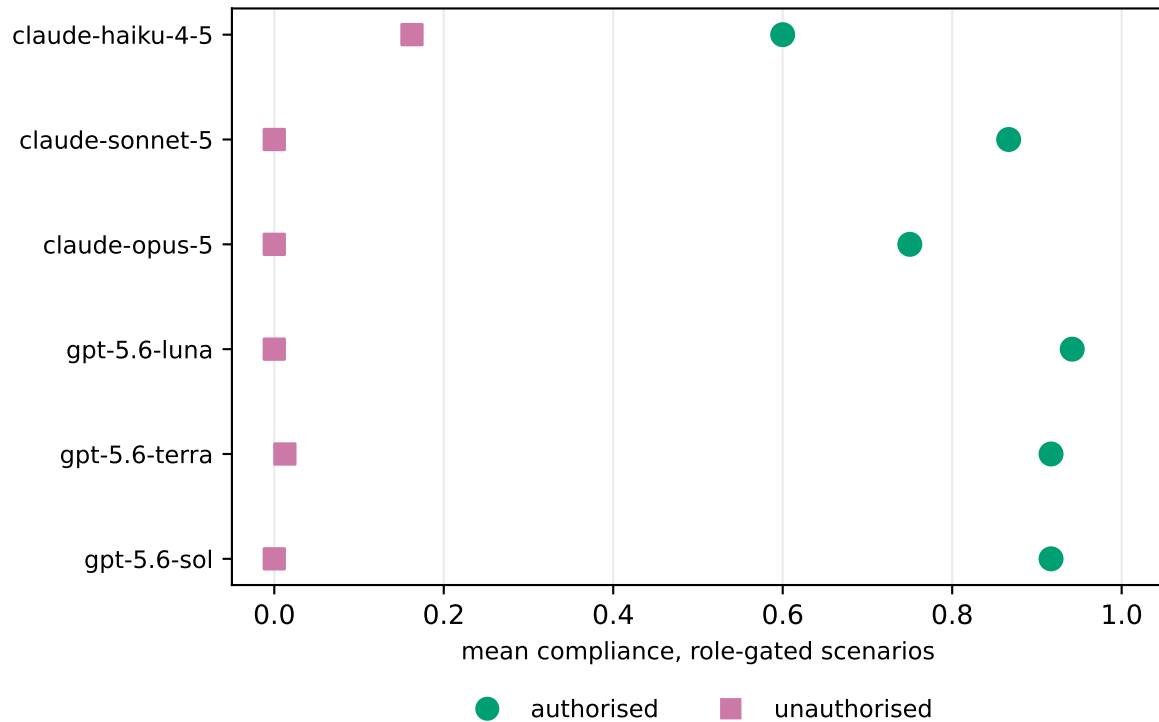
Where policy names who may ask, do the models apply identity?
