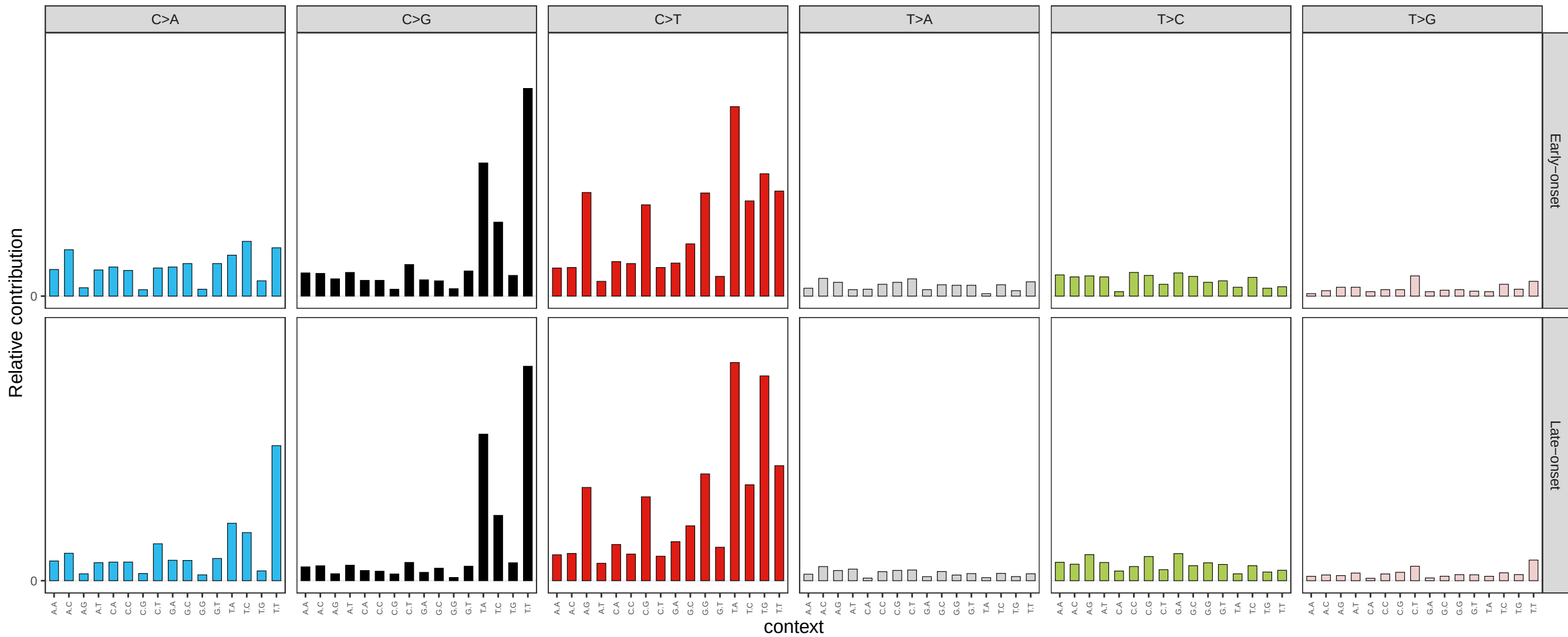
96-Channel Trinucleotide Mutation Spectrum by Onset Group
