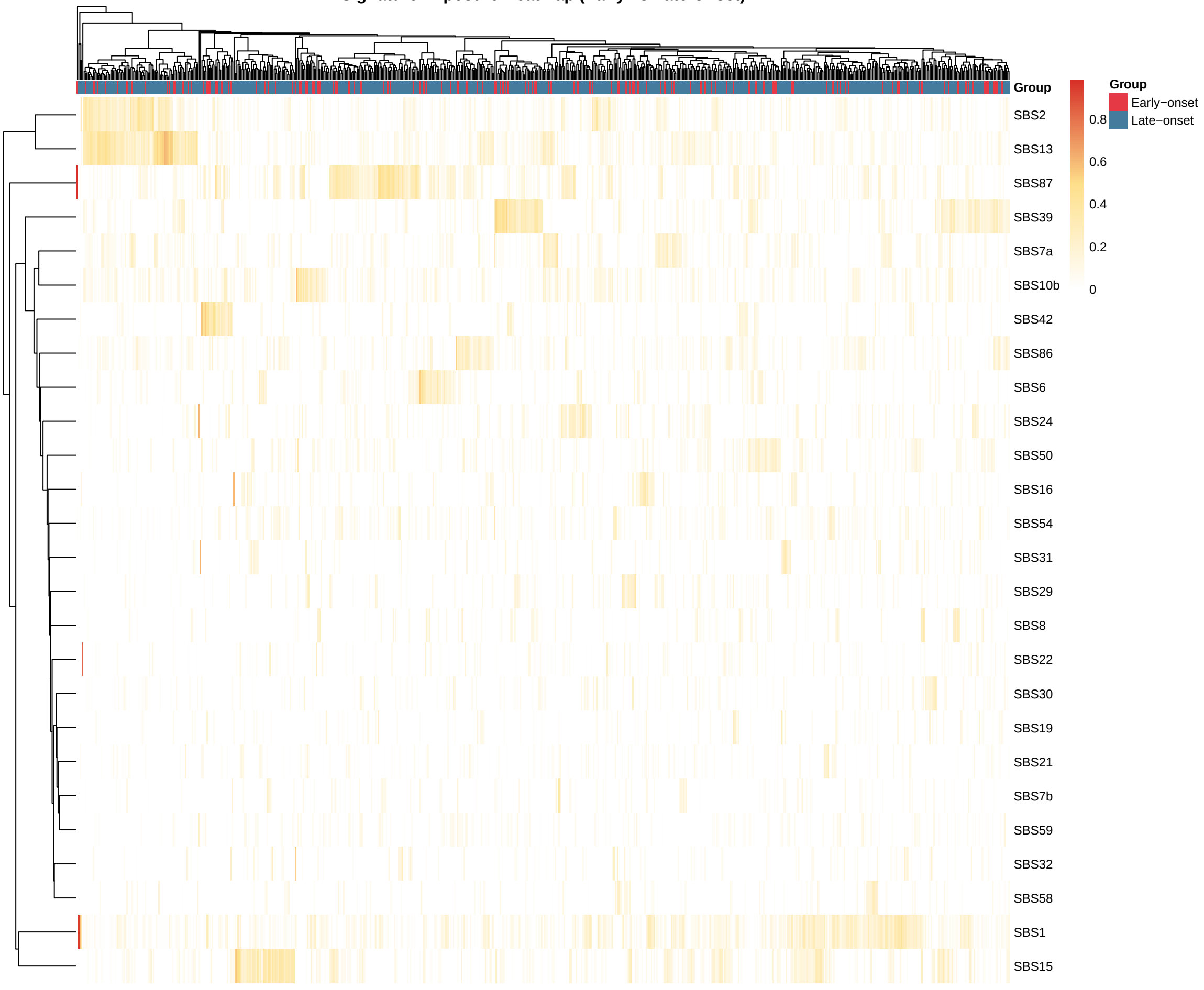
Signature Exposure Heatmap (Early vs Late Onset)
