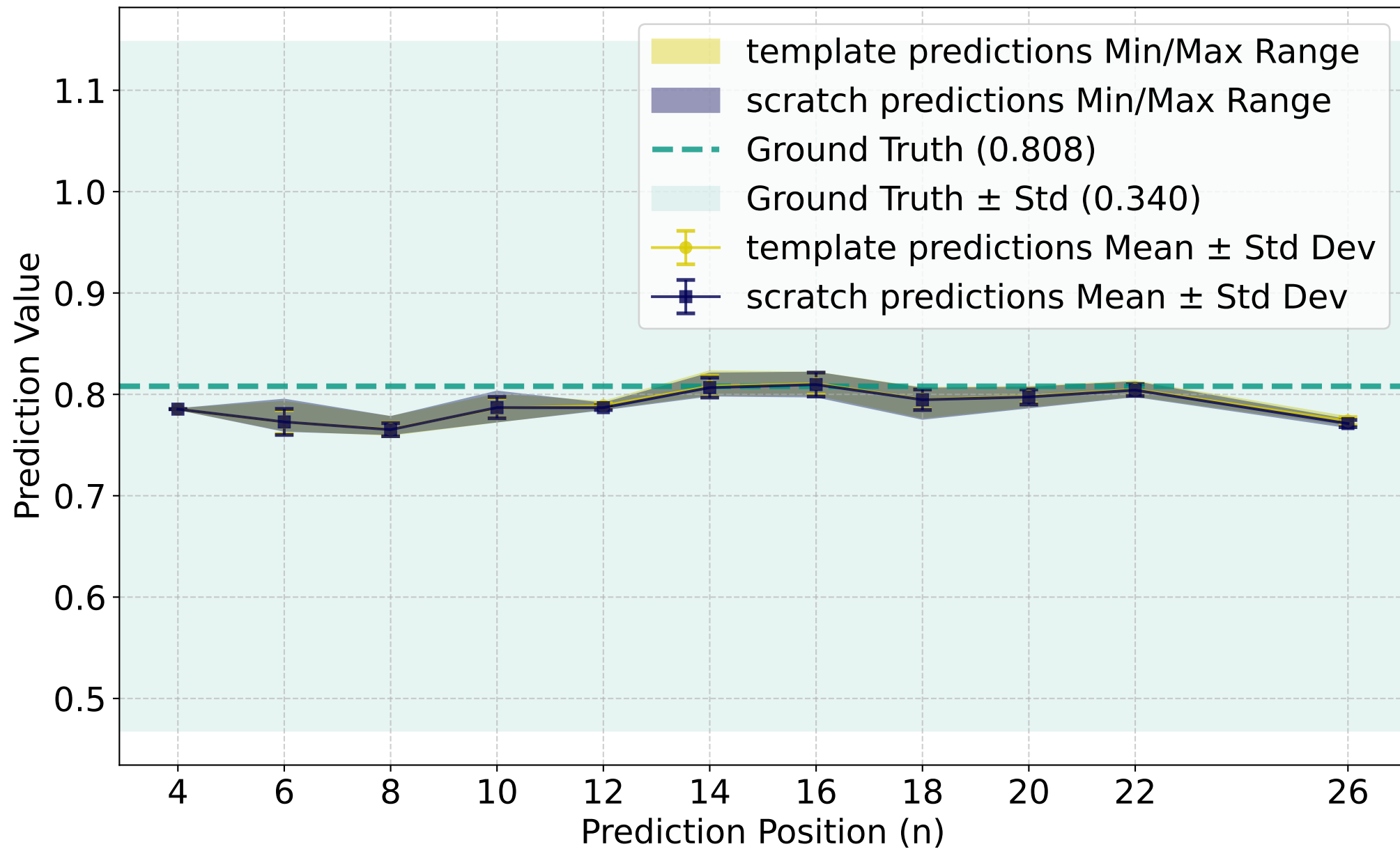
Predictions vs. Ground Truth
