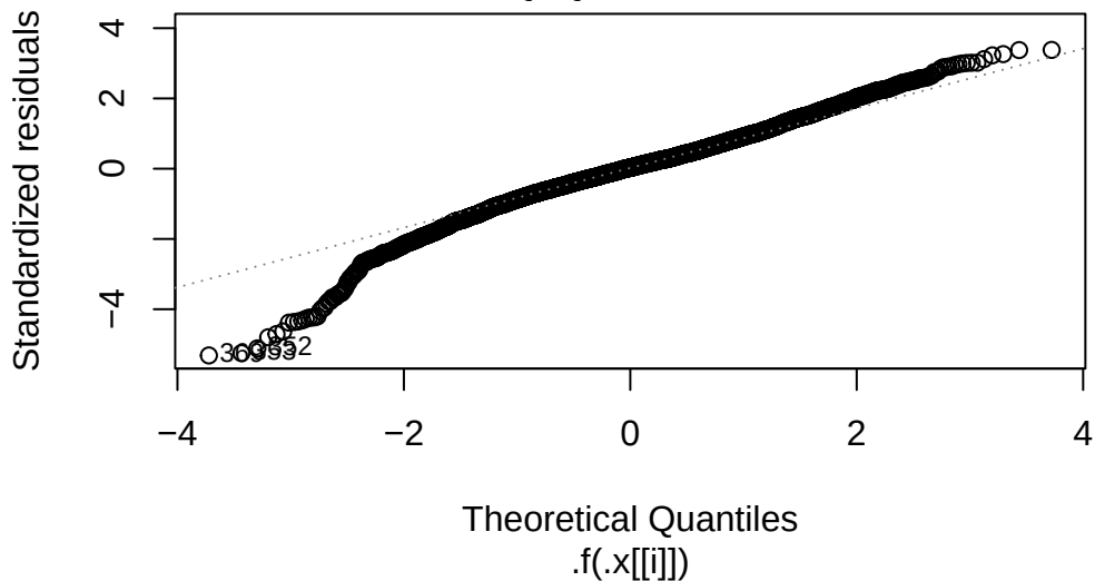
Q-Q Residuals
