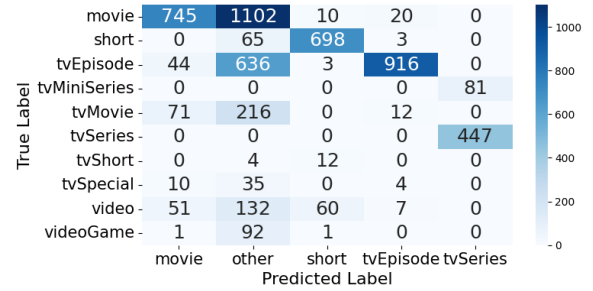
Figure 41: Confusion Matrix for rule-based classifier (10 True × 5 Predicted).
