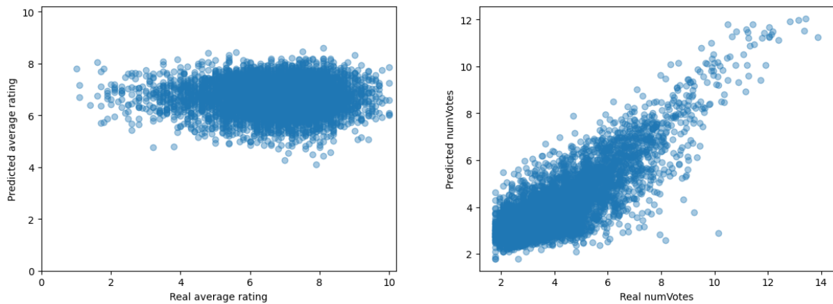
Figure 36: Relationship between real and predicted values of average rating (KNN regressor).
