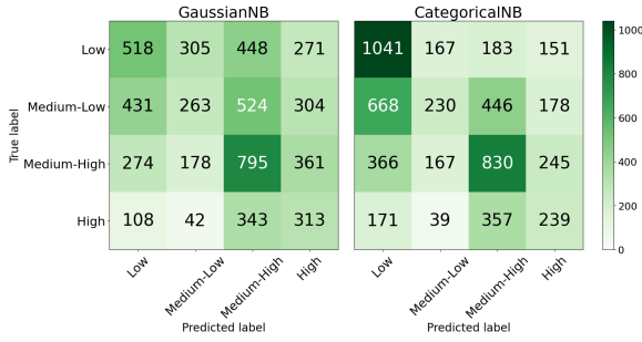
Figure 21: Confusion matrixes for GaussianNB and CategoricalNB for binned rating .
