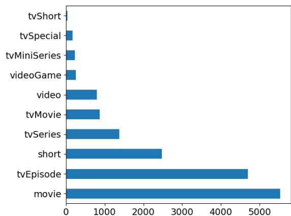
Figure 2: Barplot for titleType.
