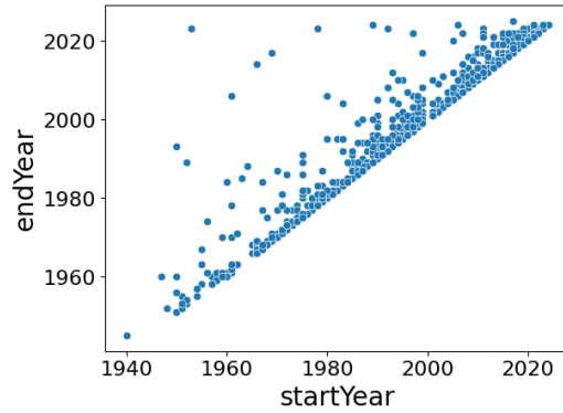
Figure 7: Scatterplot endYear ~ startYear .
