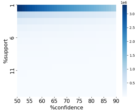
Figure 27: N. of association rules extracted for different minsup and minconf values.
