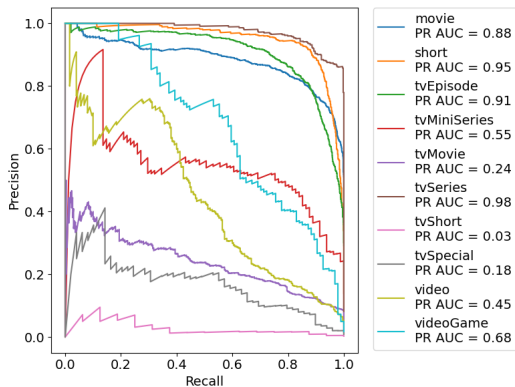
Figure 20: PR curves (1-vs-rest) for CategoricalNB.
