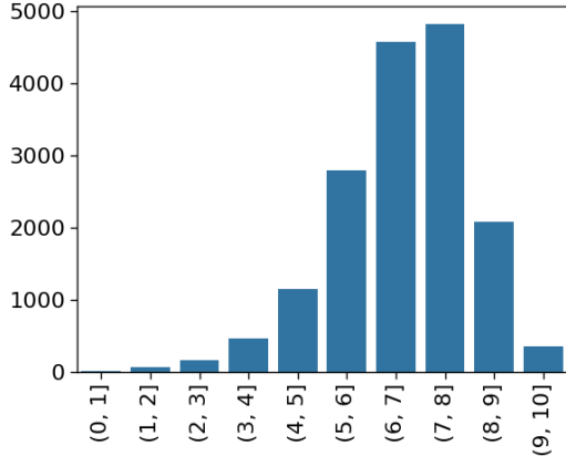
Figure 5: Barplot for rating .
