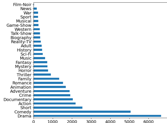
Figure 4: Barplot for genres .
