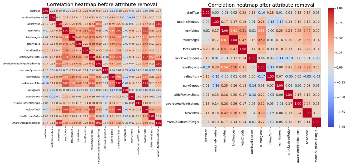
Figure 10: Correlation heatmaps, before and after attribute removal.
