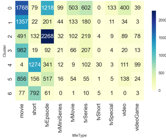
Figure 13: Heatmap Clusters vs titleType for K-Means.
