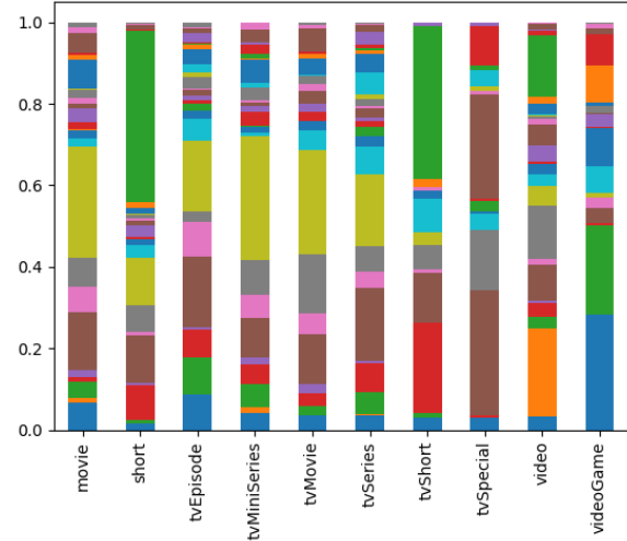
Figure 9: Title type frequency grouped by genre.
