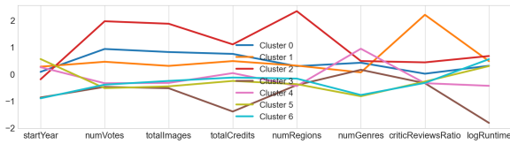
Figure 16: Centroids' visualization for BK-Means.
