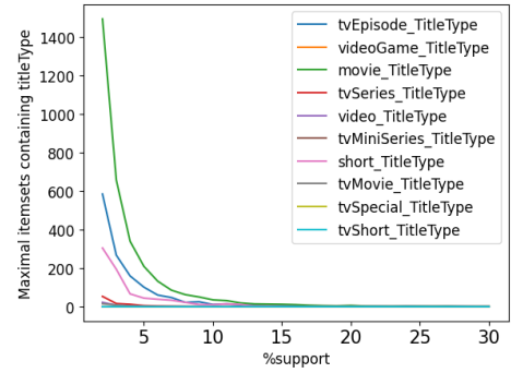
Figure 26: N. of maximal frequent itemsets containing titleType for different minsup values.
