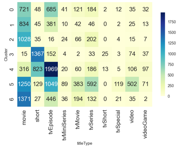
Figure 17: Heatmap Clusters vs titleType (BK-Means).
