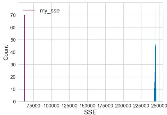
Figure 11: Statistical framework for clusters' validity: SSE (K-Means).
