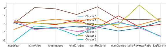
Figure 12: Centroids' visualization for K-Means.
