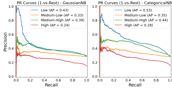
Figure 22: PR curves for GaussianNB and CategoricalNB for binned rating .
