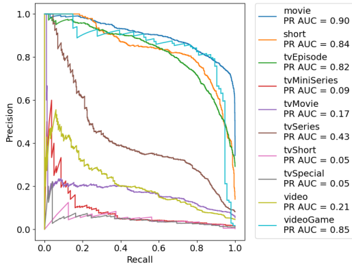
Figure 19: PR curves (1-vs-rest) for GaussianNB.
