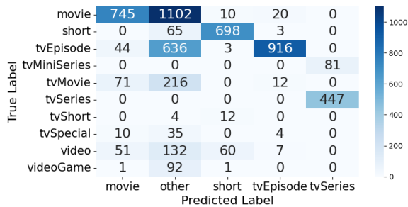
Figure 29: Confusion Matrix for rule-based classifier (10 True × 5 Predicted).
