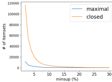
Figure 25: N. of closed and maximal frequent itemsets for different minsup values.
