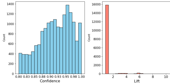
Figure 28: Histograms of rules' confidence and lift.
