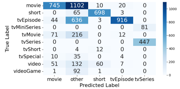
Figure 34: Confusion Matrix for rule-based classifier (10 True × 5 Predicted).
