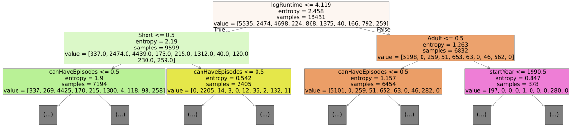
Figure 28: All-features DT for titleType , max_depth=2 (left= True, right= False).
