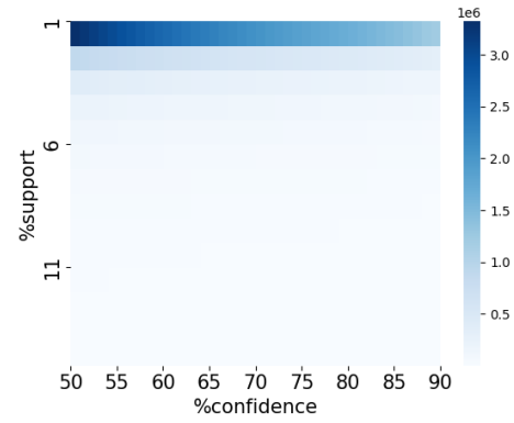
Figure 32: N. of association rules extracted for different minsup and minconf values.
