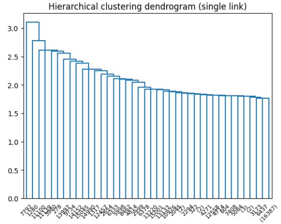
Figure 17: Dendrogram for hierarchical clustering obtained with single linkage.
