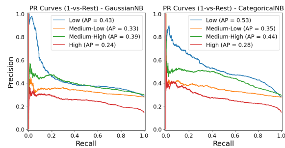
Figure 27: PR curves for GaussianNB and CategoricalNB for binned rating .
