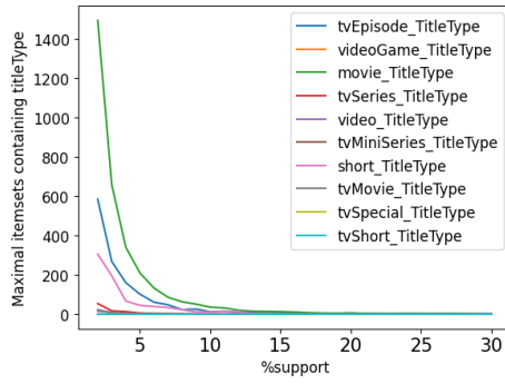
Figure 31: N. of maximal frequent itemsets containing titleType for different minsup values.
