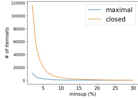
Figure 30: N. of closed and maximal frequent itemsets for different minsup values.
