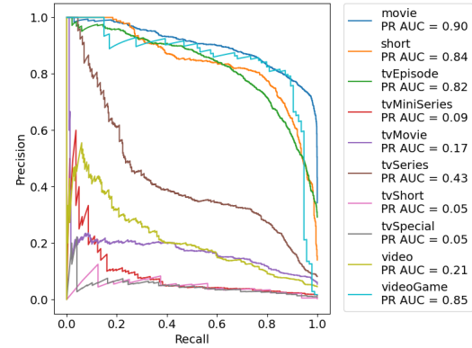
Figure 24: PR curves (1-vs-rest) for GaussianNB.
