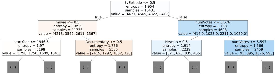
Figure 29: All-features DT for binned rating , max_depth=2 (left= True, right= False).
