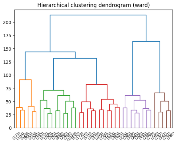
Figure 20: Dendrogram for hierarchical clustering obtained with Ward method (threshold 100).
