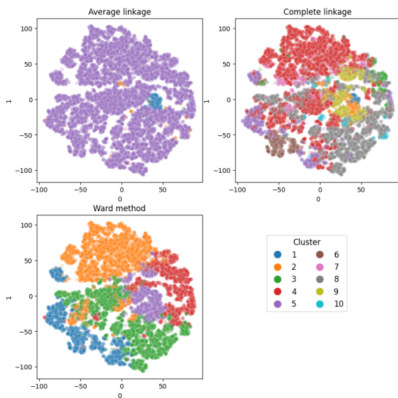
Figure 21: Clusters obtained with different criteria. Visualized by tSNE.
