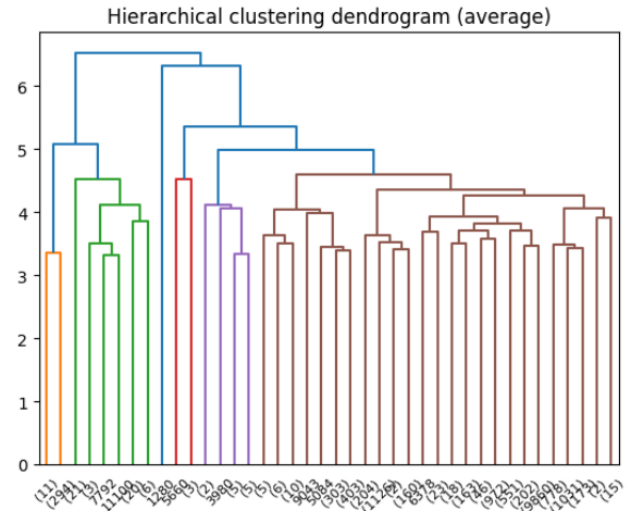
Figure 18: Dendrogram for hierarchical clustering obtained with average linkage (threshold 4.7).
