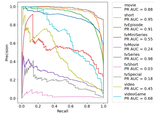
Figure 25: PR curves (1-vs-rest) for CategoricalNB.
