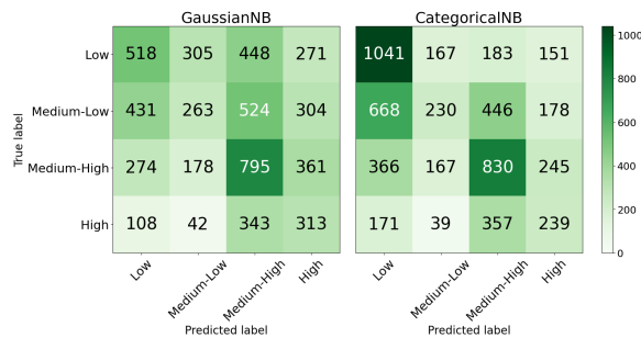
Figure 26: Confusion matrixes for GaussianNB and CategoricalNB for binned rating .
