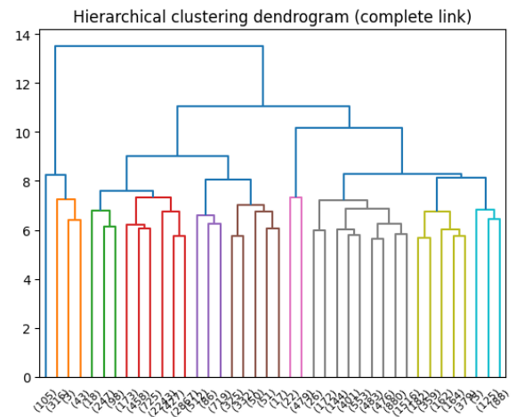
Figure 19: Dendrogram for hierarchical clustering obtained with complete linkage (threshold 7.5).
