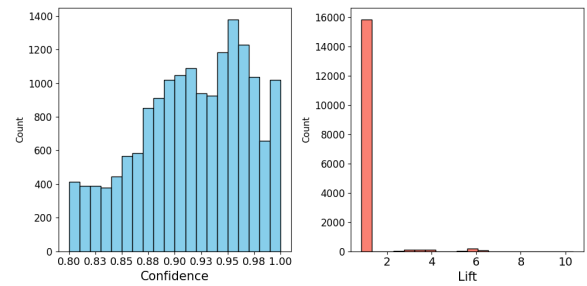
Figure 33: Histograms of rules' confidence and lift.
