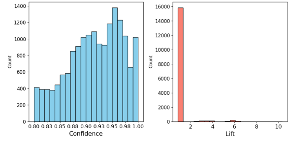
Figure 39: Histograms of rules' confidence and lift.
