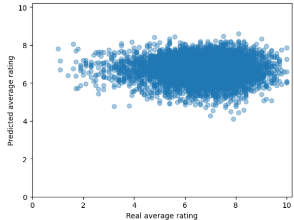
Figure 35: Relationship between real and predicted values of average rating (KNN regressor).
