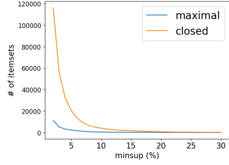
Figure 36: N. of closed and maximal frequent itemsets for different minsup values.
