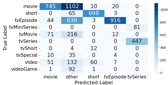
Figure 40: Confusion Matrix for rule-based classifier (10 True × 5 Predicted).
