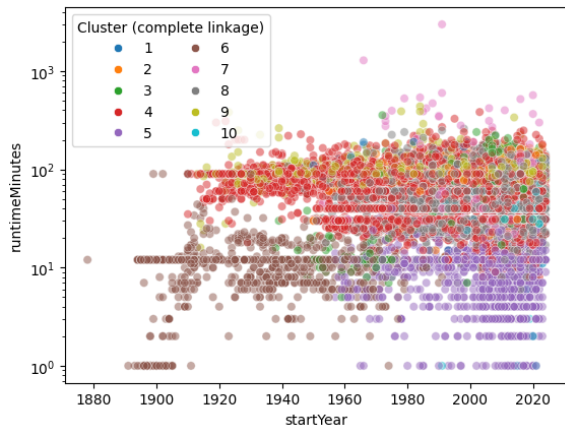
Figure 24: Complete linkage clustering by year of release and runtime.
