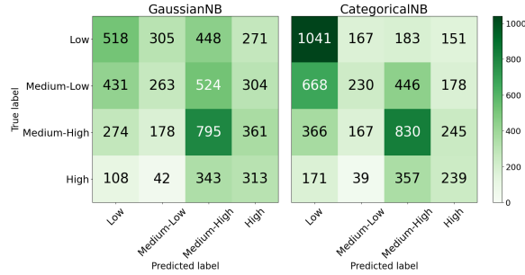
Figure 31: Confusion matrices for GaussianNB and CategoricalNB for binned rating .
