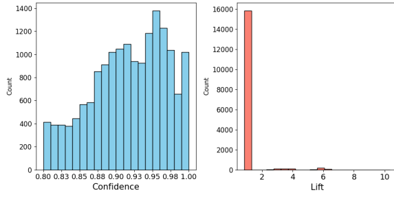
Figure 39: Histograms of rules' confidence and lift.
