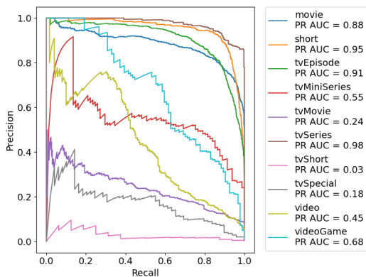
Figure 30: PR curves (1-vs-rest) for CategoricalNB.
