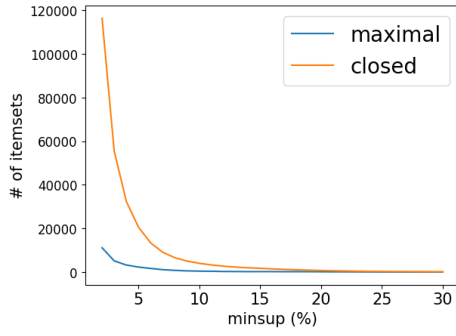
Figure 36: N. of closed and maximal frequent itemsets for different minsup values.
