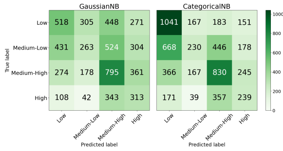
Figure 31: Confusion matrixes for GaussianNB and CategoricalNB for binned rating .
