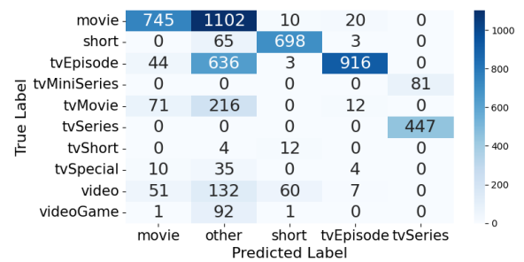
Figure 39: Confusion Matrix for rule-based classifier (10 True × 5 Predicted).
