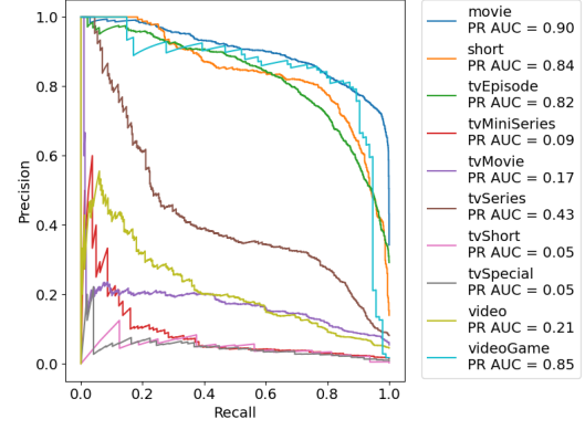
Figure 29: PR curves (1-vs-rest) for GaussianNB.
