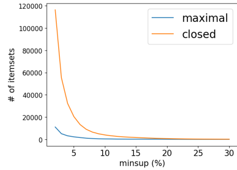
Figure 35: N. of closed and maximal frequent itemsets for different minsup values.
