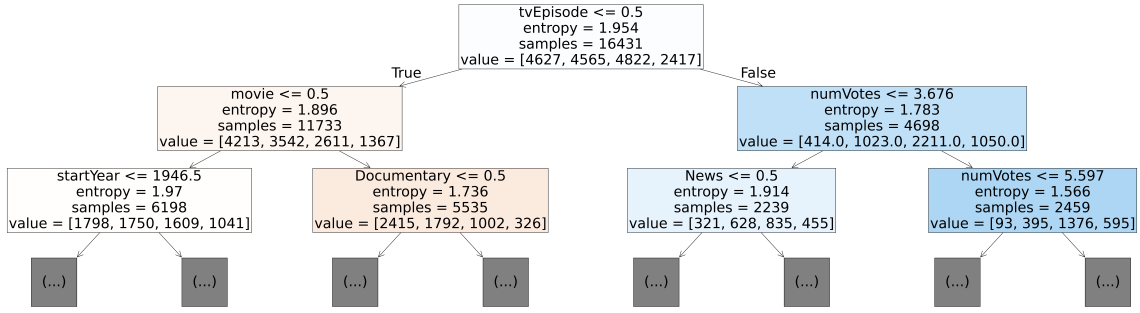
Figure 22: All-features DT for binned rating , max_depth=2 (left= True, right= False).
