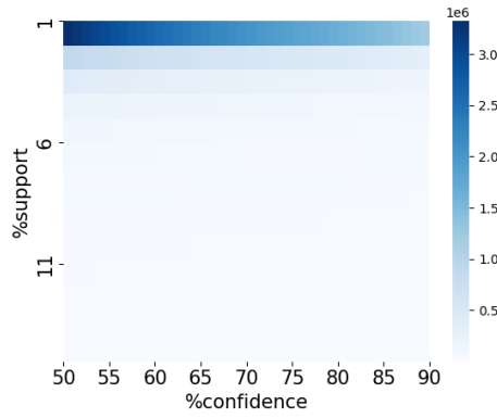
Figure 25: N. of association rules extracted for different minsup and minconf values.
