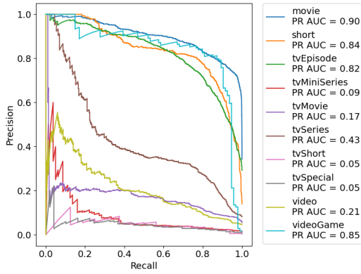
Figure 17: PR curves (1-vs-rest) for GaussianNB.
