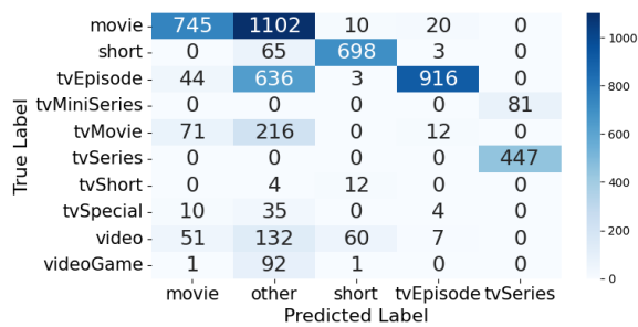
Figure 27: Confusion Matrix for rule-based classifier (10 True × 5 Predicted).
