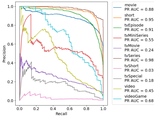
Figure 18: PR curves (1-vs-rest) for CategoricalNB.
