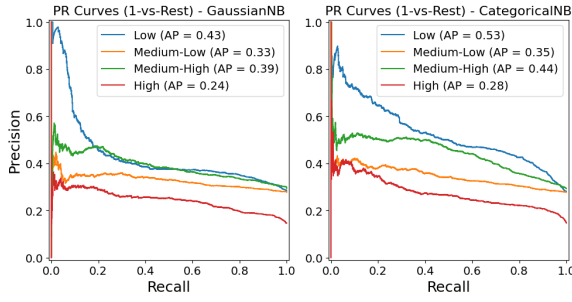
Figure 20: PR curves for GaussianNB and CategoricalNB for binned rating .
