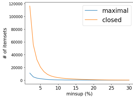
Figure 23: N. of closed and maximal frequent itemsets for different minsup values.
