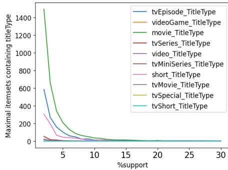
Figure 24: N. of maximal frequent itemsets containing titleType for different minsup values.
