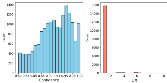
Figure 26: Histograms of rules' confidence and lift.
