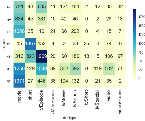
Figure 15: Heatmap Clusters vs titleType (BK-Means).
