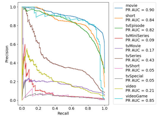
Figure 22: PR curves (1-vs-rest) for GaussianNB.
