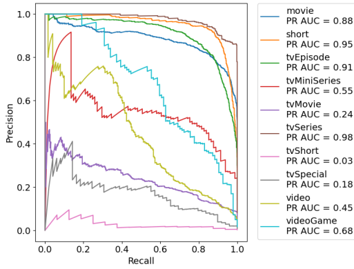
Figure 23: PR curves (1-vs-rest) for CategoricalNB.
