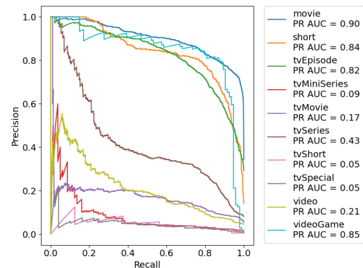
Figure 20: PR curves (1-vs-rest) for GaussianNB.
