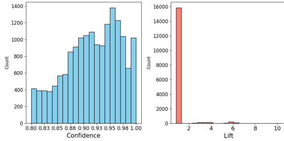
Figure 27: Histograms of rules' confidence and lift.
