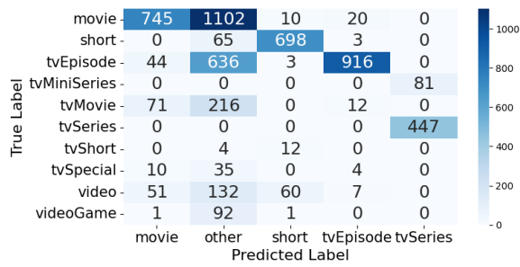
Figure 28: Confusion Matrix for rule-based classifier (10 True \times 5 Predicted).
