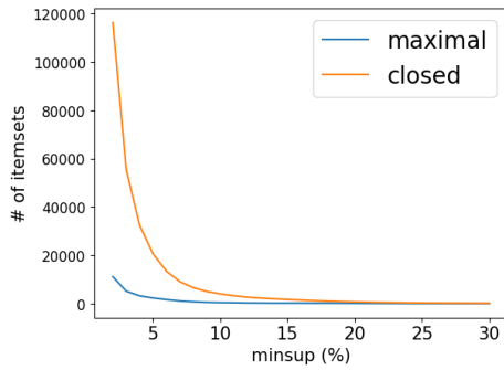
Figure 24: N. of closed and maximal frequent itemsets for different minsup values.
