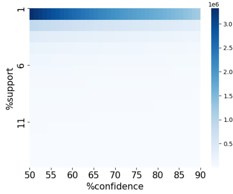
Figure 26: N. of association rules extracted for different minsup and minconf values.
