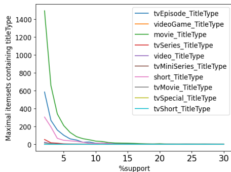
Figure 25: N. of maximal frequent itemsets containing titleType for different minsup values.
