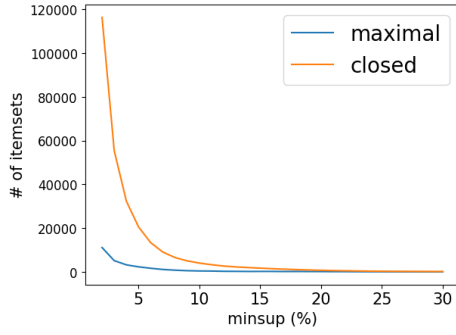
Figure 26: N. of closed and maximal frequent itemsets for different minsup values.
