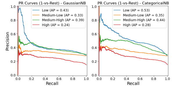
Figure 23: PR curves for GaussianNB and CategoricalNB for binned rating .
