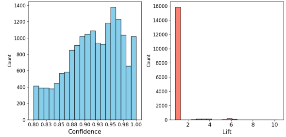
Figure 29: Histograms of rules' confidence and lift.
