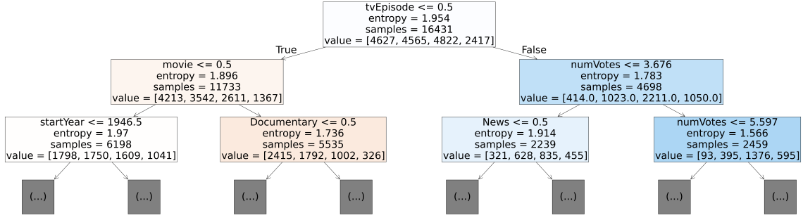
Figure 25: All-features DT for binned rating , max_depth=2 (left= True, right= False).
