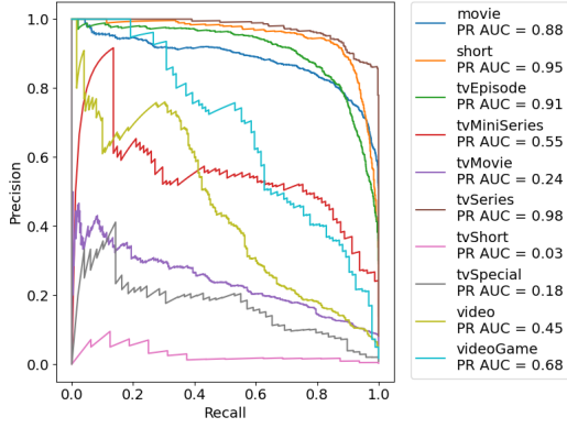
Figure 21: PR curves (1-vs-rest) for CategoricalNB.
