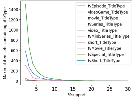
Figure 27: N. of maximal frequent itemsets containing titleType for different minsup values.
