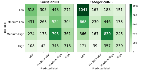
Figure 22: Confusion matrixes for GaussianNB and CategoricalNB for binned rating .
