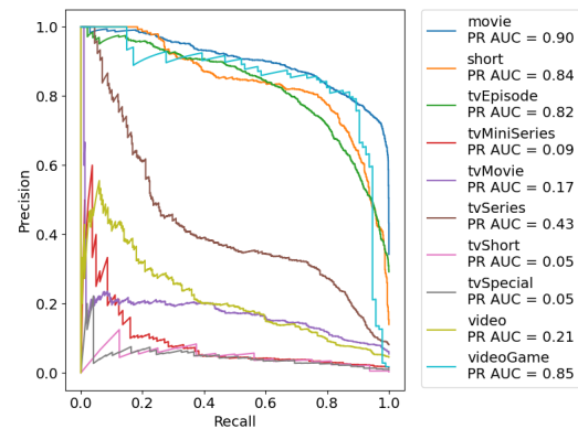
Figure 20: PR curves (1-vs-rest) for GaussianNB.
