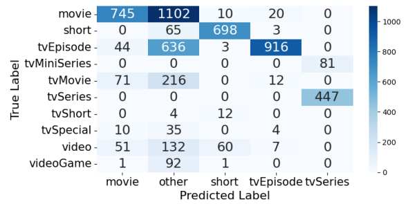
Figure 30: Confusion Matrix for rule-based classifier (10 True × 5 Predicted).
