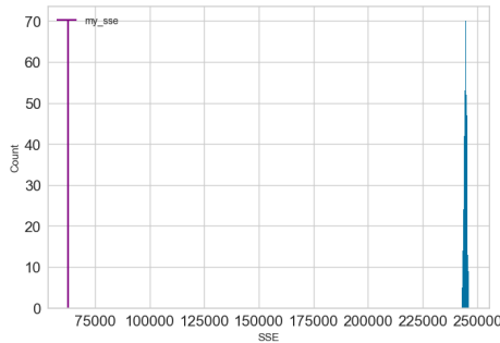
Figure 12: Statistical framework for clusters' validity: see (K-Means).
