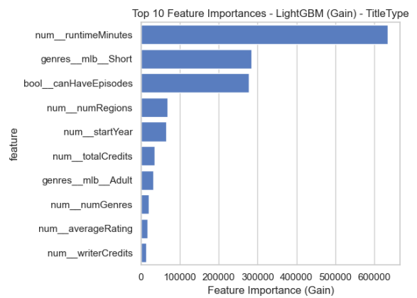
Figure 16: Top 10 most important features for titleType (LightGBM).
