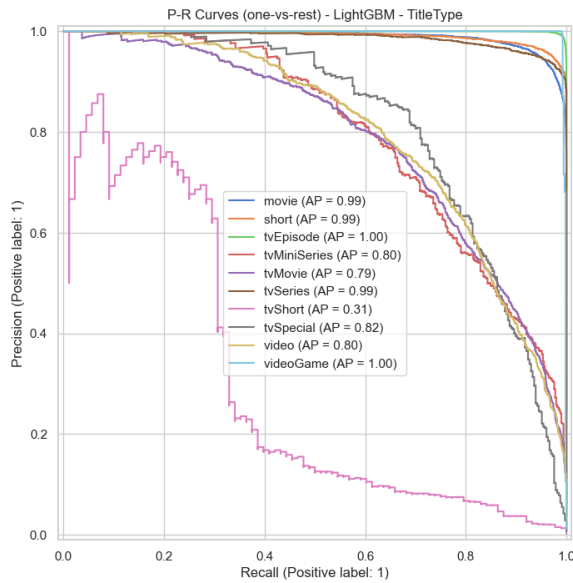
Figure 18: PR curves for titleType (LightGBM).
