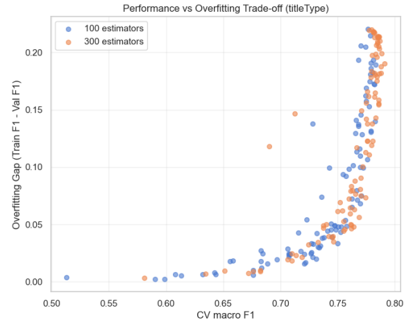
Figure 17: Trade-off between avg validation macro F1 and overfitting gap for titleType (LightGBM).
