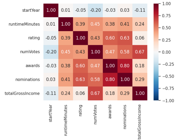
Figure 29: Correlation of numeric features.
