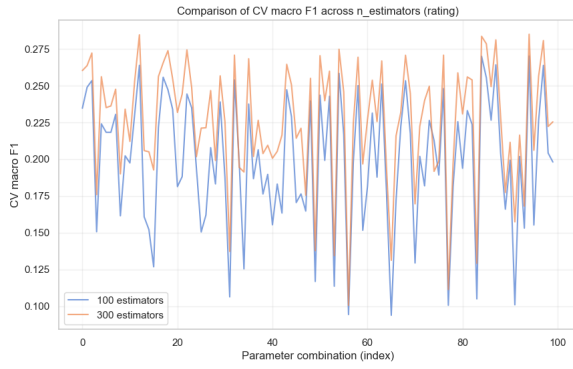
Figure 14: Avg. cross-validation macro F1 for different parameter configurations for 100 and 300 DTs for rating (LightGBM).
