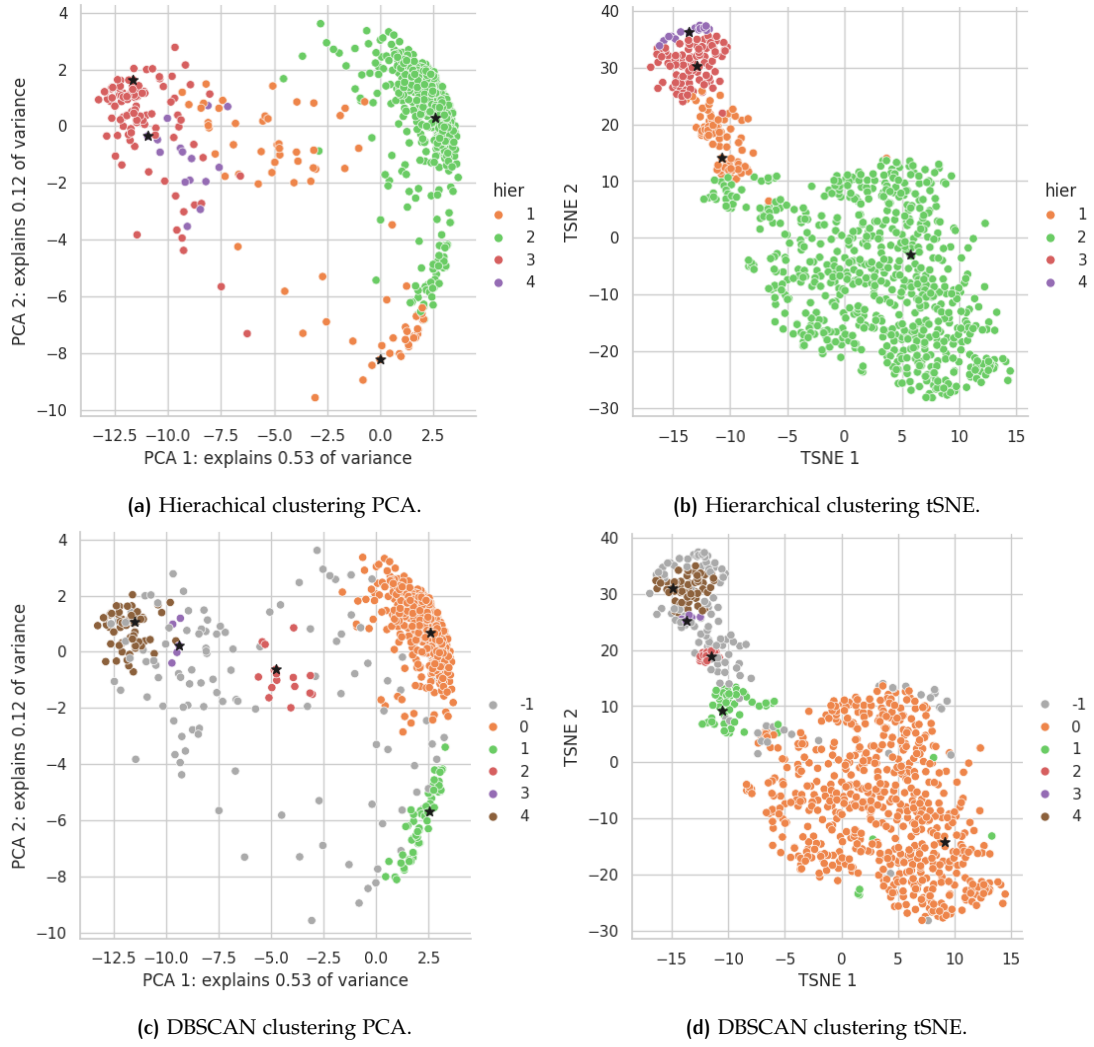
Figure 34: Clusters and cluster medoids for hierarchical clustering and DBSCAN visualized with two dimensionality reduction techniques.
