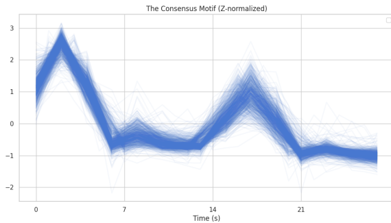
Figure 39: Best match for the consensus motif on all time series.
