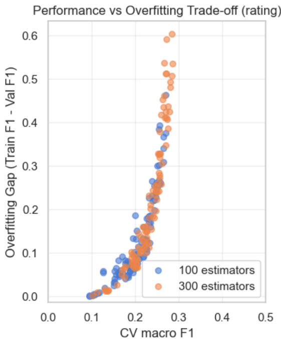
Figure 16: Trade-off between avg validation macro F1 and overfitting gap for rating (LightGBM).
