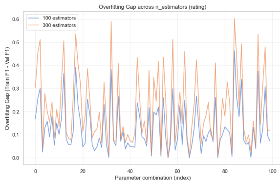
Figure 15: Overfitting gap for different parameter configurations for 100 and 300 DTs for rating (LightGBM).
