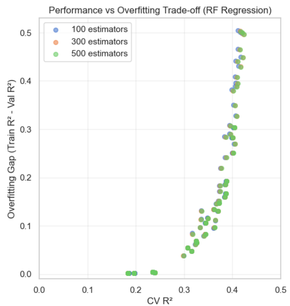
Figure 24: Trade-off between avg validation R^2 and overfitting gap for averageRating (RF Regressor).
