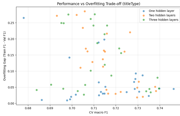
Figure 21: Trade-off between validation macro F1 and overfitting gap for titleType (MLP).
