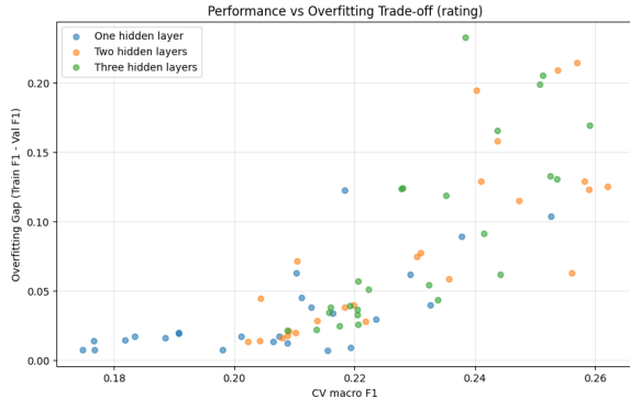
Figure 20: Trade-off between validation macro F1 and overfitting gap for rating (MLP).
