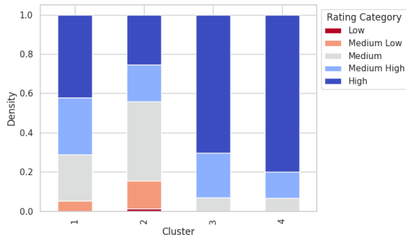
Figure 35: Distribution of binned rating by cluster (hierarchical).
