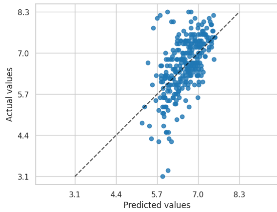
Figure 44: Relationship between real ratings and rating predicted by the C22 regressor during testing.
