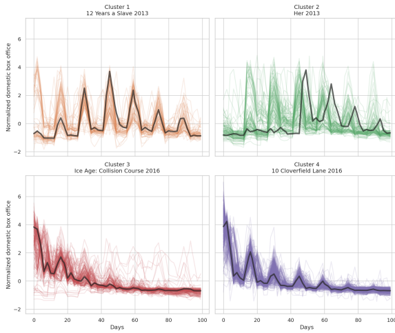
Figure 36: Clusters obtained by hierarchical clustering on structural features and respective cluster medoids (in black).
