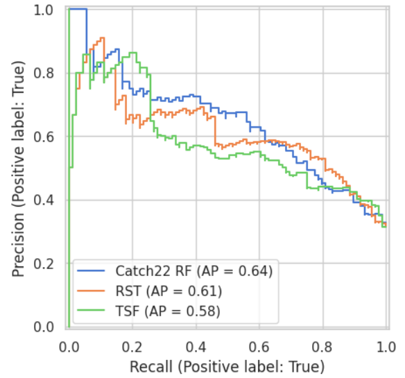
Figure 42: Precision-Recall curves for the action classification task on test set.
