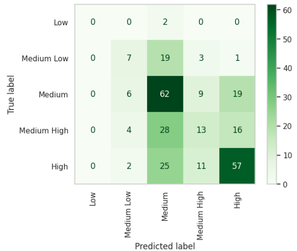
Figure 43: Confusion matrix for C22 classifier on the test set.
