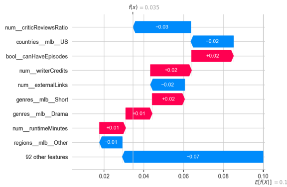
Figure 23: Waterfall plot for medoid n. 11 for its correct label tvMovie (3.5% confidence).
