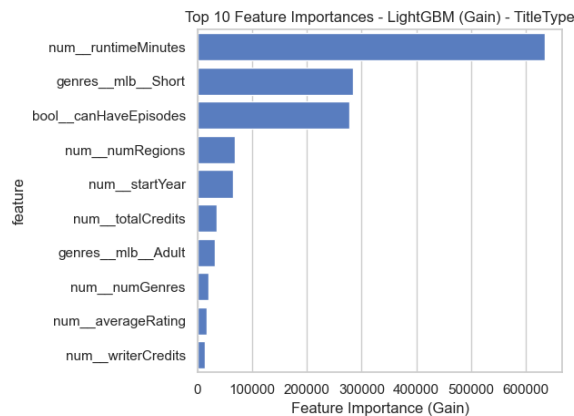
Figure 19: Top 10 most important features for titleType (LightGBM).
