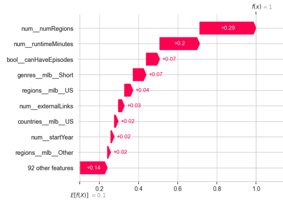
Figure 22: Waterfall plot for medoid n. 5 (correct tvEpisode , 100% confidence).
