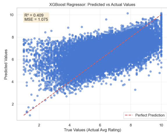
Figure 27: Relationship between real and predicted values of averageRating (XGBoost Regressor).
