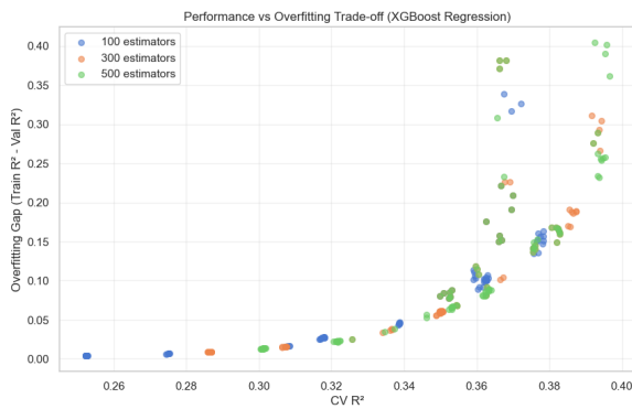
Figure 26: Trade-off between avg validation R2 and overfitting gap for averageRating (XGBoost Regressor).
