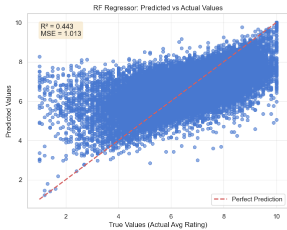
Figure 25: Relationship between real and predicted values of averageRating (RF Regressor).
