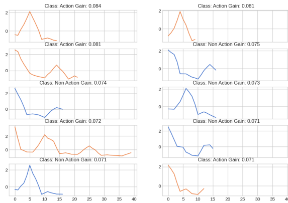
Figure 40: Shapelets extracted by Random Shapelet Transformer (shapelets for the positive class in orange).
