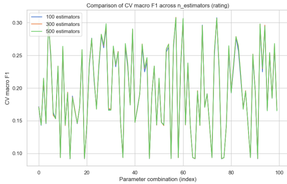
Figure 10: Avg cross-validation macro F1 for different parameter configurations across varying numbers of estimators for rating (RF).
