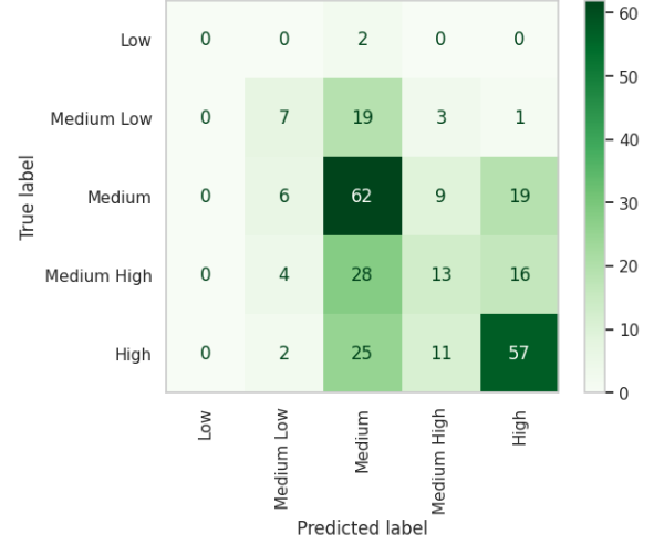
Figure 43: Confusion matrix for C22 classifier on the test set.
