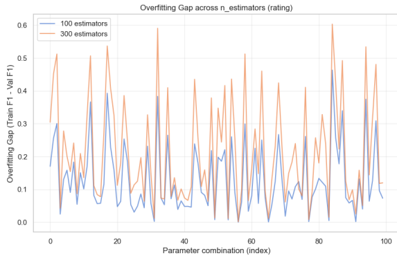
Figure 15: Overfitting gap for different parameter configurations for 100 and 300 DTs for rating (LightGBM).
