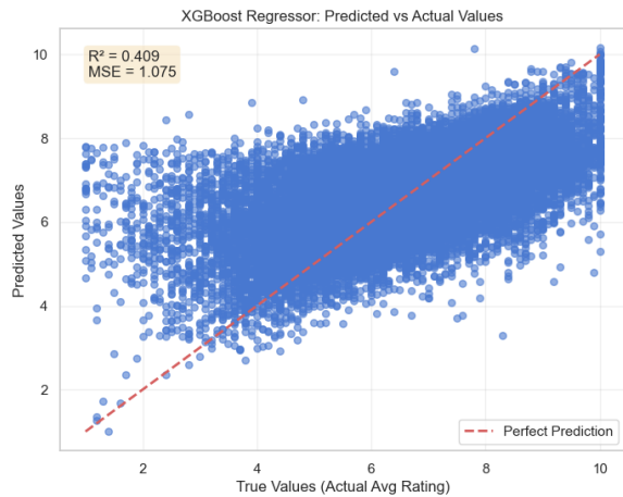
Figure 24: Relationship between real and predicted values of averageRating (XGBoost Regressor).
