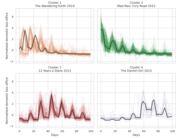
Figure 29: Clusters obtained by hierarchical clustering and respective cluster medoids (in black).
