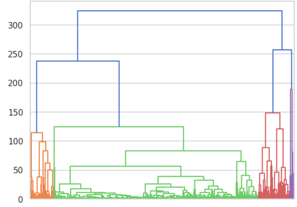
Figure 28: Dendrogram for shape-based hierarchical clustering.
