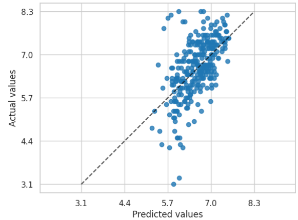
Figure 41: Relationship between real ratings and rating predicted by the C22 regressor during testing.
