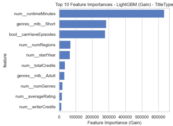
Figure 16: Top 10 most important features for titleType (LightGBM).
