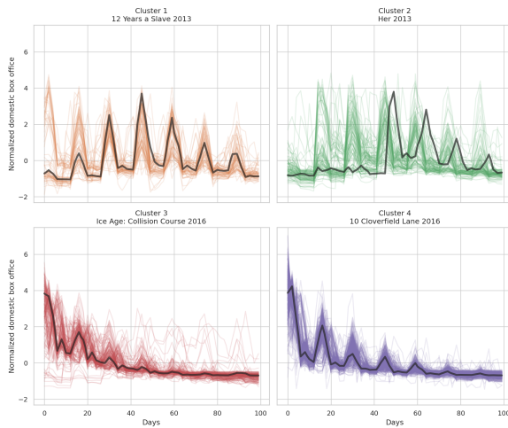
Figure 33: Clusters obtained by hierarchical clustering on structural features and respective cluster medoids (in black).
