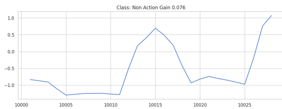
Figure 38: Shapelet extracted from Matrix Profile.
