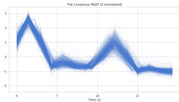
Figure 36: Best match for the consensus motif on all time series.
