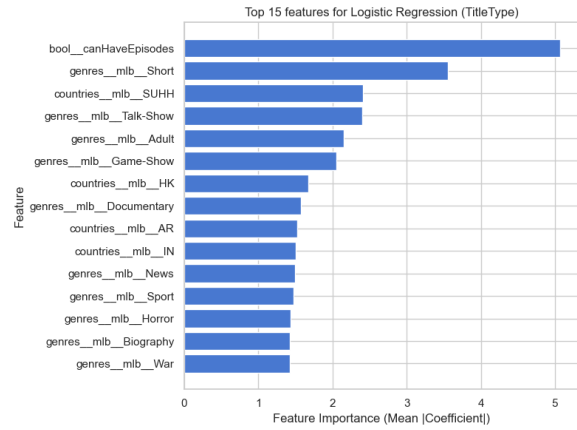
Figure 6: Top 15 most important features for titleType
