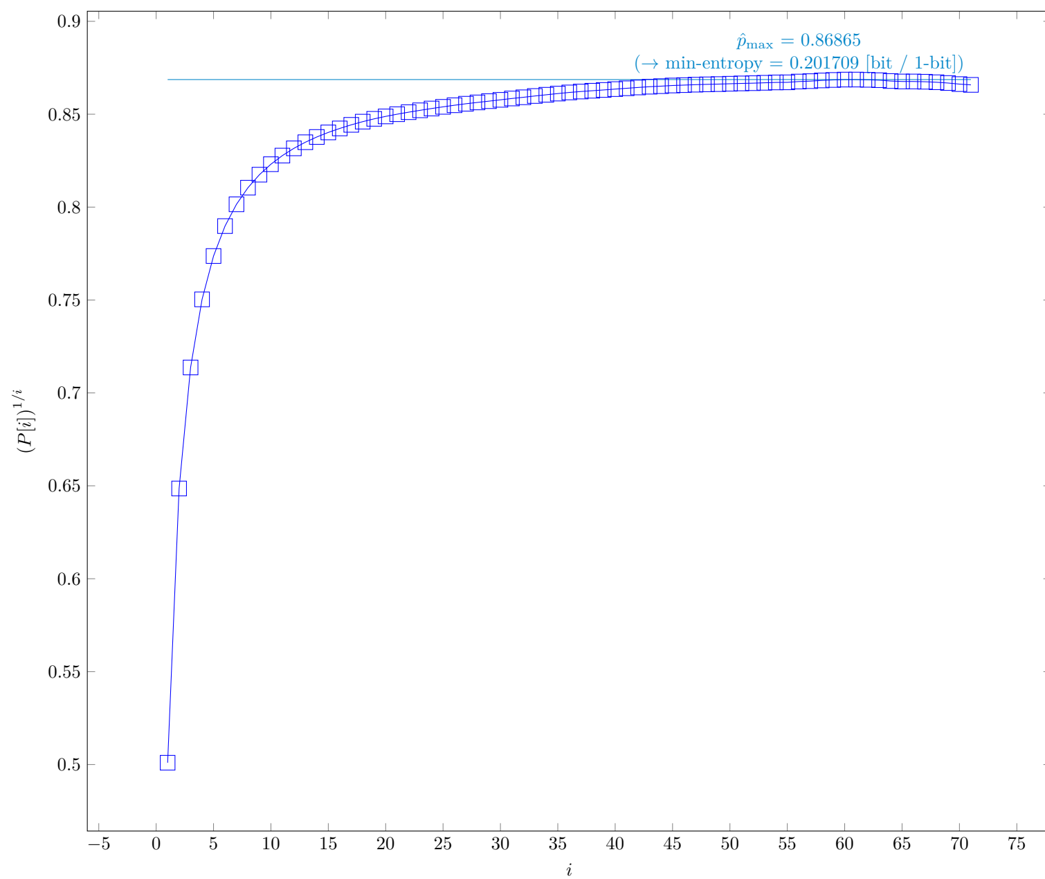
Fig. 9 P[i]^{1/i} in §6.3.5 of NIST SP 800-90B
