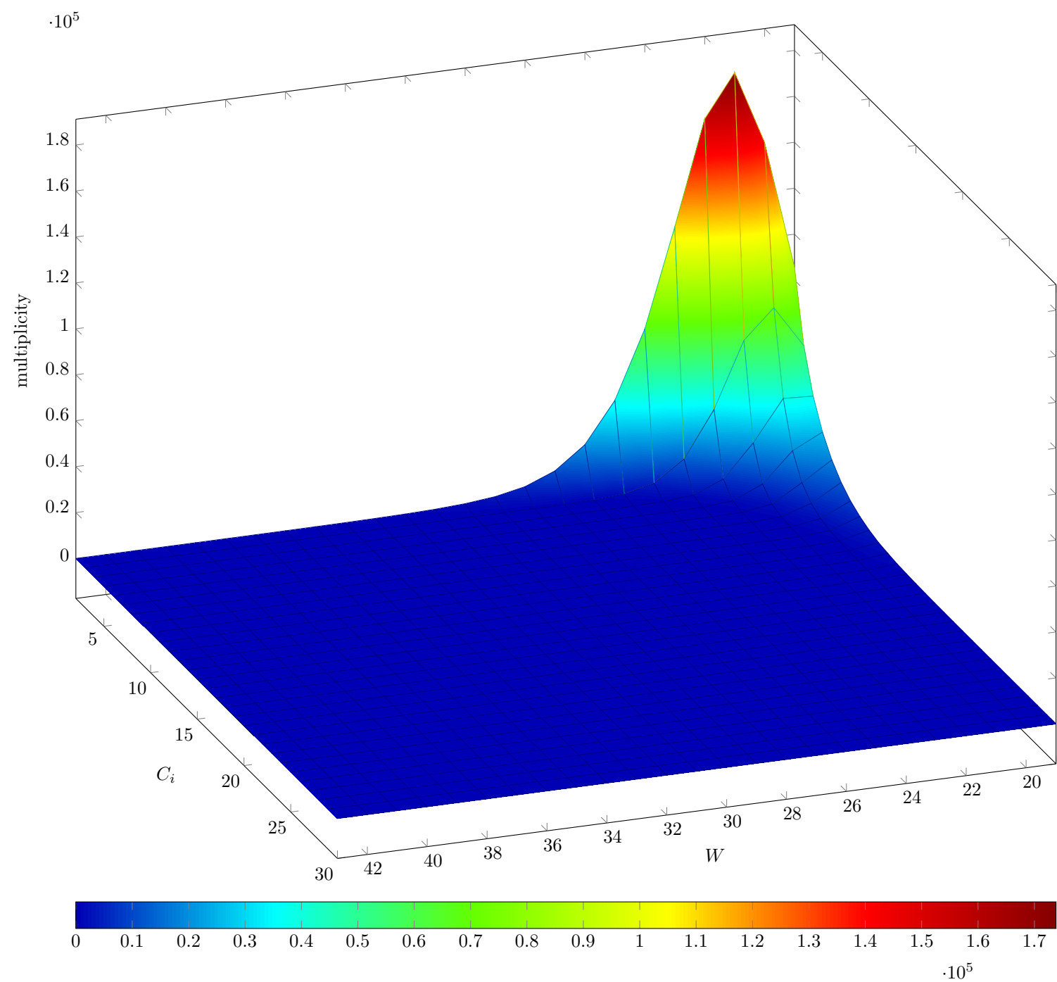
Fig. 10 Distribution of the multiplicity of W -tuple having the same C_i value in Step 3 of §6.3.6 of NIST SP 800-90B
