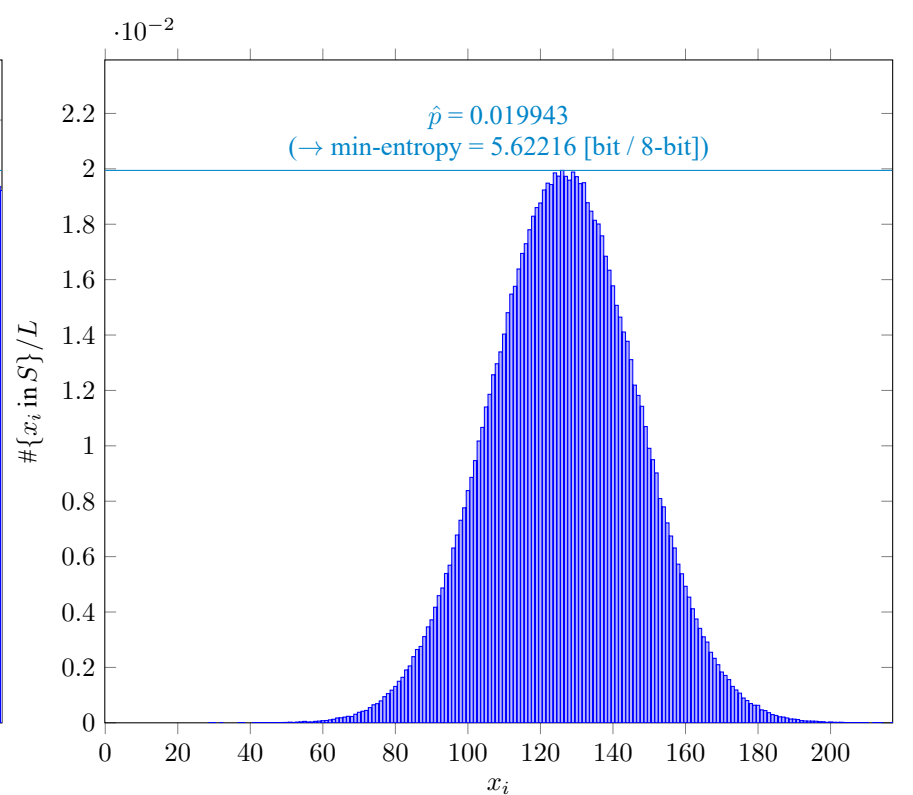
Fig. 4 Distribution of x_i for normal.bin [7]
