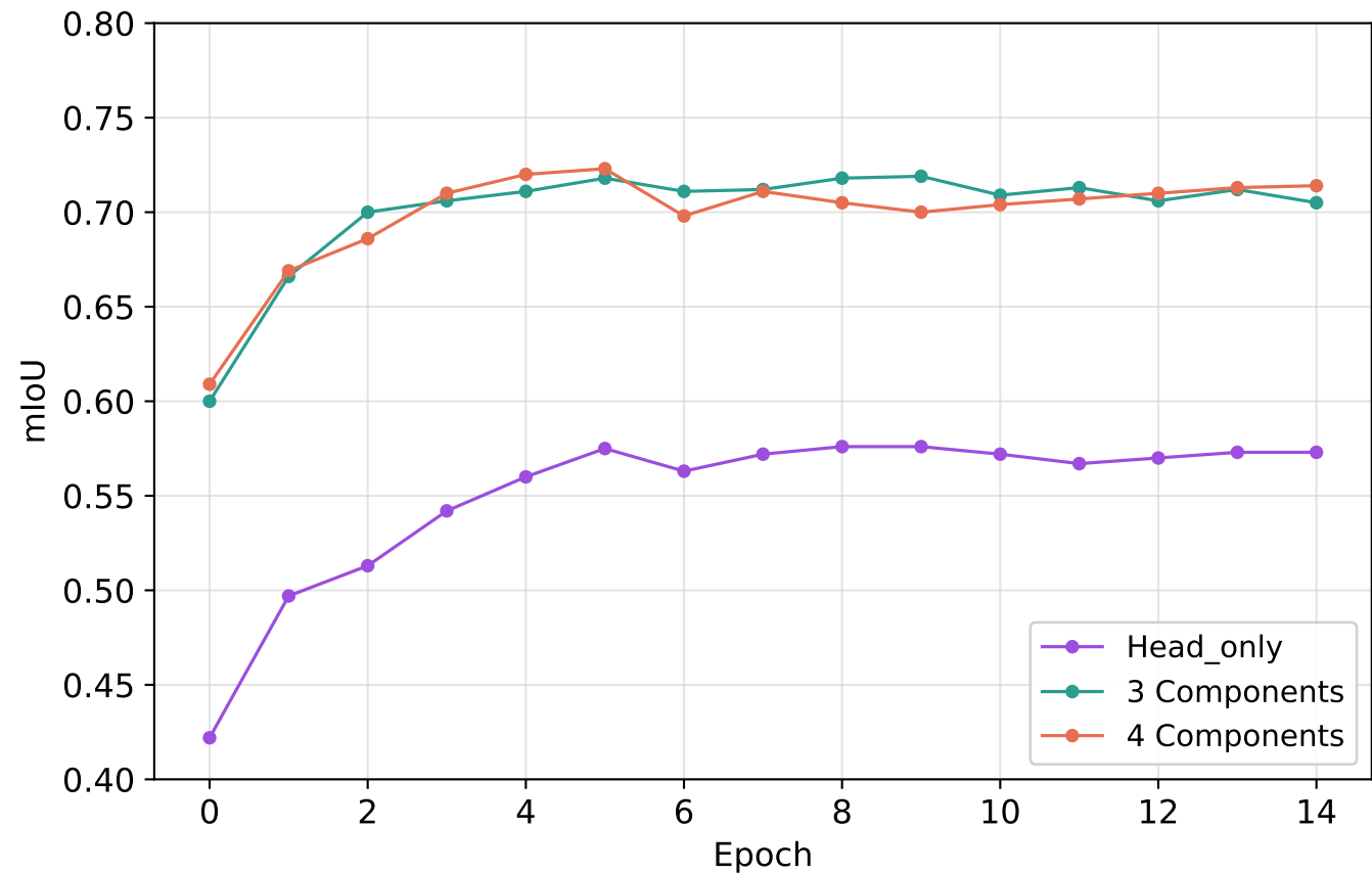
EoMT Fine-Tuning comparison
