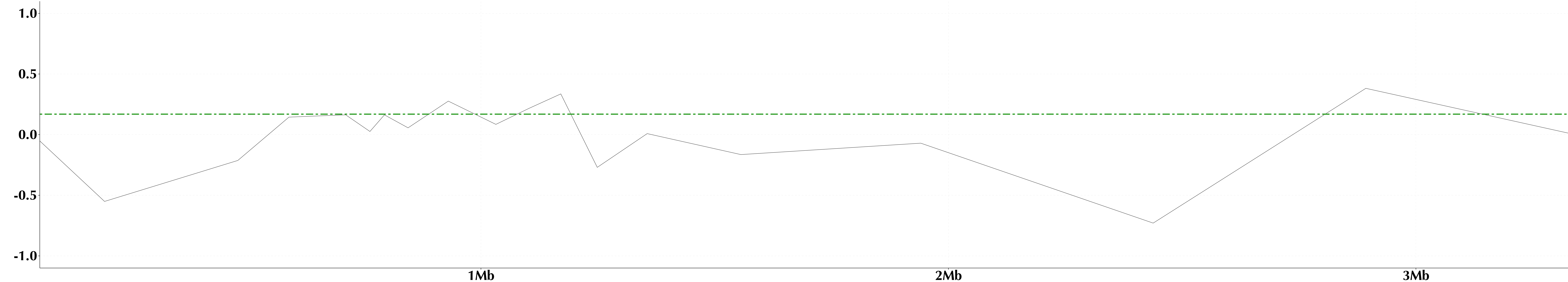
Genomic Position
