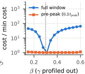
(b) profile likelihood
