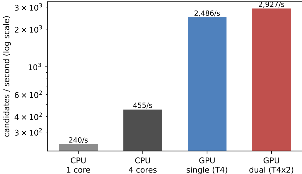
PBKDF2-HMAC-SHA1 throughput: CPU vs GPU (Kaggle T4x2)
