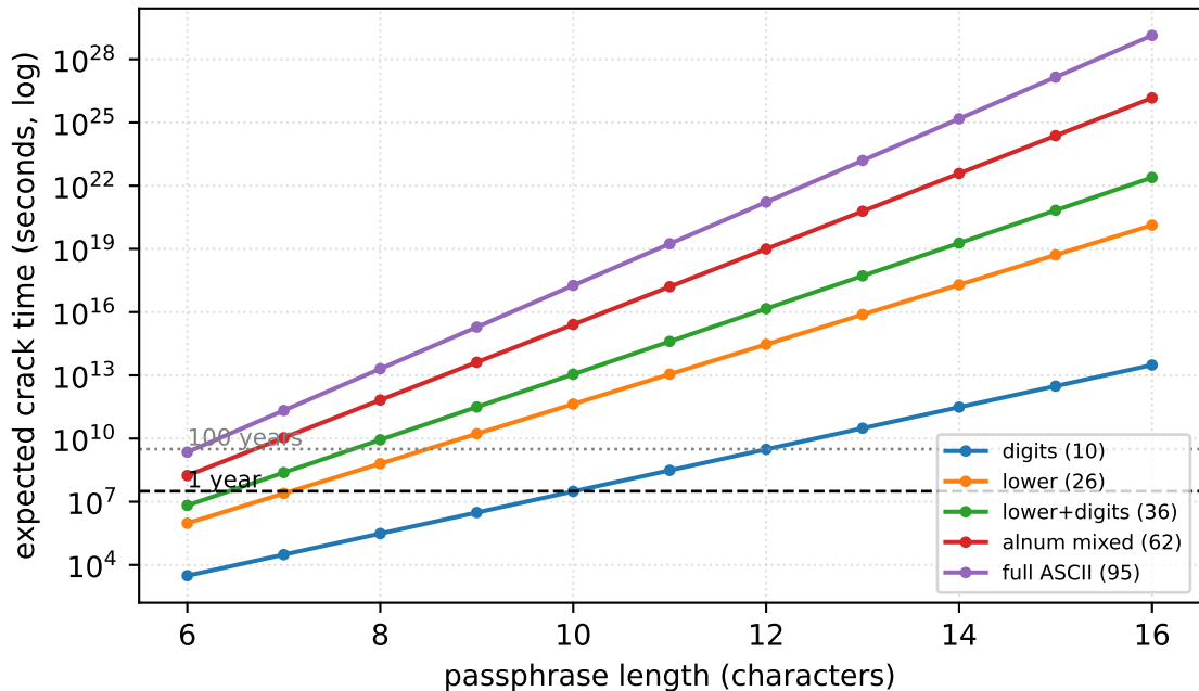
Offline crack time vs length @ 162 cand/s
